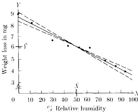
FIGURE 11.10 95% confidence limits to regression line of Figure 11.6.
