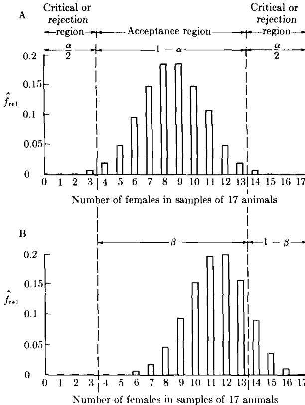
FIGURE 6.8 Expected distributions of outcomes when sampling 17 animals from two hypothetical populations. (A) H_0: p_i = q_j = \frac{1}{2} ; (B) H_1: p_i = 2q_j = \frac{2}{3} . Dashed lines separate critical regions from acceptance region of the distribution of part A. Type I error \alpha equals approximately 0.01.
