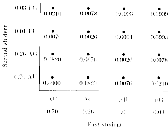
FIGURE 4.1 Sample space for sampling two students from Matchless University.
