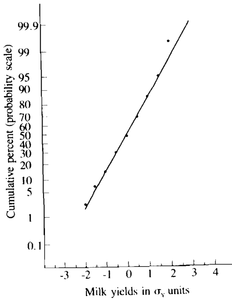
FIGURE 6.2 Graphic analysis of means of 1400 random samples of 5 milk yields and of means of 200 random samples of 35 milk yields.
