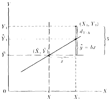
FIGURE 11.9 Schematic diagram to show relations involved in partitioning the sum of squares of the dependent variable.
