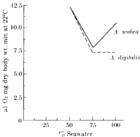
FIGURE 9.2 Oxygen consumption by two species of limpets at three salinities. Data from Box 9.1.
