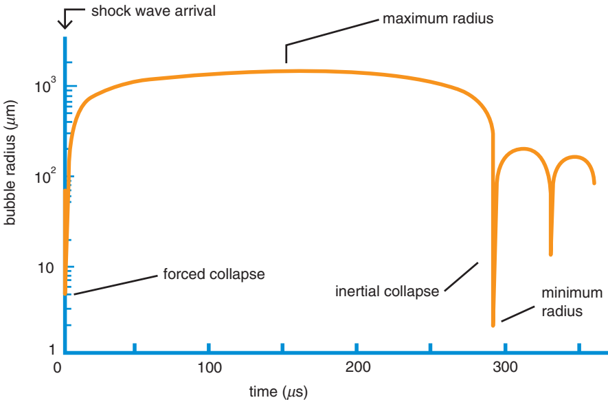
Fig. 4.8 Graph of a numerical simulation showing the variation of the radius of an air bubble in water (initial radius R_0=0.07\ \text{mm} ) exposed to a lithotripter shock wave ( p^+=100\ \text{MPa} ). An abrupt forced bubble collapse is followed by an expansion and a second collapse. The second collapse occurred approximately 290\ \mu\text{s} after arrival of the shock wave at t=0 . The bubble rebounds several times (not shown completely) until reaching equilibrium. (Courtesy of M. de Icaza-Herrera)
