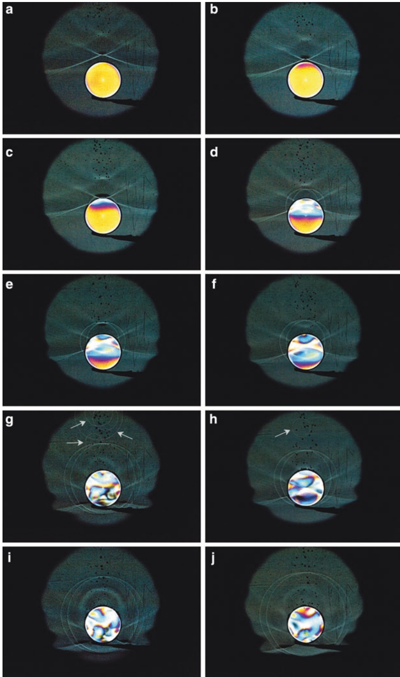
Fig. 3.17 Photographic sequence of an underwater shock wave hitting an acrylic cylinder (20 mm in diameter) from the top of the images, showing the reflected waves in different phases. The colors ( eBook ) display a stress pattern inside the cylinder. Secondary shock waves generated by shock wave-induced bubble collapse can be observed in images (g) and (h) (see arrows ). Cavitation bubbles are distinguished as black dots . Technique: schlieren optics in combination with photoelastic stress imaging (Photographs: O. Wess and J. Mayer, Storz Medical AG, Tägerwilten, Switzerland)
