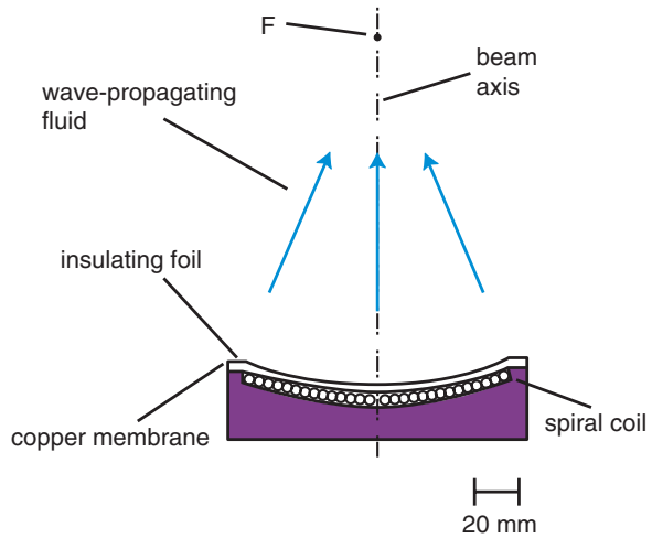
Fig. 5.53 Schematic of a self-focusing electromagnetic shock wave source
