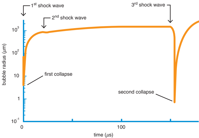
Fig. 4.14 Graph of a numerical simulation showing the variation of the radius of an air bubble in water (initial radius R_0=0.07 mm) exposed to the pressure profile shown in Fig. 4.13. The second collapse occurred approximately 155 \mu\text{s} after arrival of the first shock wave at t=0 . (Courtesy of M. de Icaza-Herrera)
