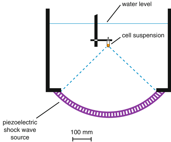
Fig. 7.10 Schematic of a setup to transflect human cells in vitro. Test vials containing cell suspensions are positioned at the focal spot of a piezoelectric shock wave source
