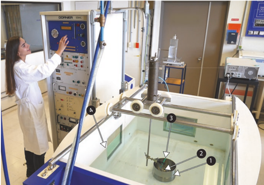
Fig. 5.5 Photograph of the electrohydraulic research shock wave generator at the Shock Wave Laboratory, Center for Applied Physics and Advanced Technology, UNAM, showing (1) the stainless steel ellipsoidal reflector, (2) the spark-plug, (3) the clamp fastened to the xyz positioner, and (4) the water level. The upper part of the control console belongs to the HM3 shock wave generator shown in Fig. 5.9, and the lower part houses the controls for the device shown here. (Photograph: F. Fernández)
