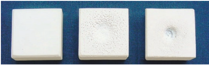
Fig. 4.5 Photograph of three (30×30×14.3 mm) AST 110 stone models (High Medical Technologies, Kreuzlingen, Switzerland), before ( left ) and after exposure to 500 underwater shock waves generated with an electrohydraulic ( center ) and a piezoelectric ( right ) shock wave source
