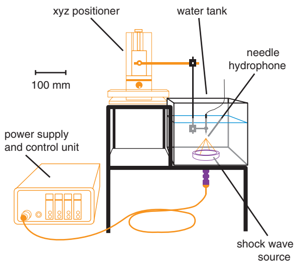
Fig. 5.59 Schematic of a Piezoson 100 plus -based research device (Richard Wolf GmbH, Knittlingen, Germany)
