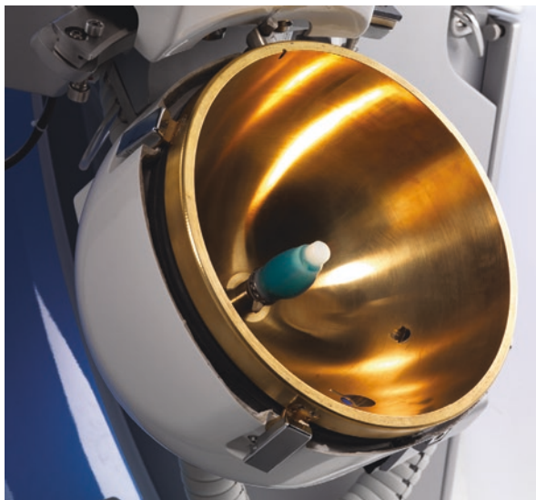
Fig. 5.24 Photograph of the ellipsoidal reflector and the electroconductive spark-plug of a Sonolith i-sys lithotripter. (Courtesy of EDAP TMS, Vaulx-en-Velin, France)
