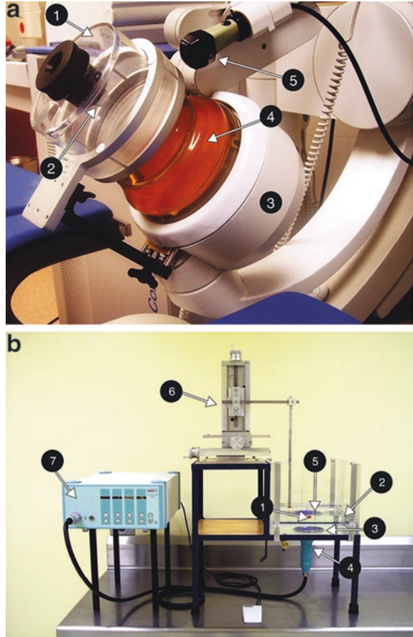
Fig. 5.11 (a) Photograph of a Compact Sigma shock wave lithotripter (Dornier MedTech GmbH, Wessling, Germany), showing (1) a small water test tank, (2) a mesh to place kidney stone phantoms inside the water tank, (3) the shock wave source, (4) the water cushion, and (5) the ultrasound scanner. (b) Photograph of an experimental device based on a Piezoson 100 Plus (Richard Wolf GmbH, Knittlingen, Germany) shock wave unit showing (1) a vial placed at the focus inside the water tank, (2) the water level, (3) the coupling membrane, (4) the shock wave source, (5) the reflection of the coupling membrane on the water surface, (6) the xyz positioner, and (7) the power supply and control unit. (Photograph: F. Fernández)
