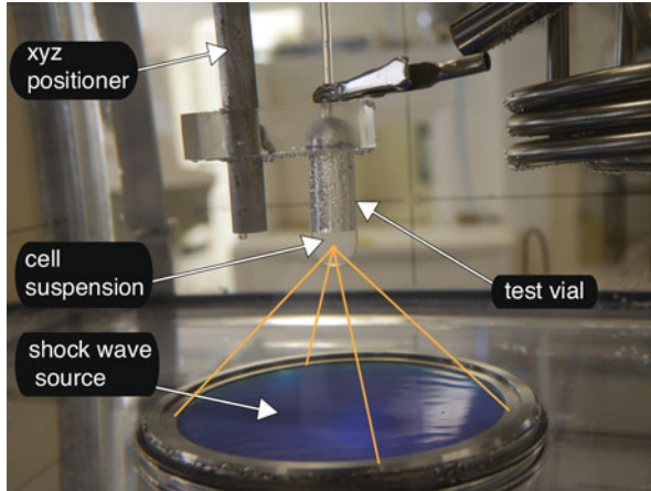
Fig. 7.8 Photograph of a Piezoson 100 -based research device (Richard Wolf GmbH, Knittlingen, Germany) used to expose cell suspensions to underwater shock waves
