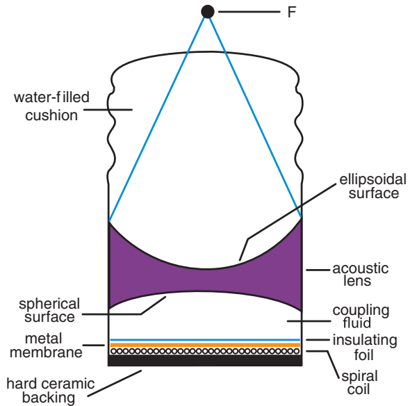
Fig. 5.41 Schematic of a flat coil electromagnetic shock wave source
