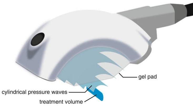
Fig. 6.10 Schematic of an FBL10x5G2 double-layer piezoelectric linear shock wave therapy source as used in the PiezoWave2 (Courtesy of Richard Wolf GmbH, Knittlingen, Germany)
