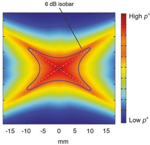
Fig. 5.52 Bi-dimensional image of the pressure distribution generated in the vicinity of the focal spot of a Duet Magna lithotripter, after simultaneously firing its two electromagnetic shock wave sources. The colors ( eBook ) represent positive peak pressure variations, according to the vertical chart at the right side of the figure. The pressure at each point inside the region bordered by the 6 dB isobar equals to 50% or more of the maximum peak-positive pressure. (Courtesy of Direx Systems Corporation, Canton MA, USA)
