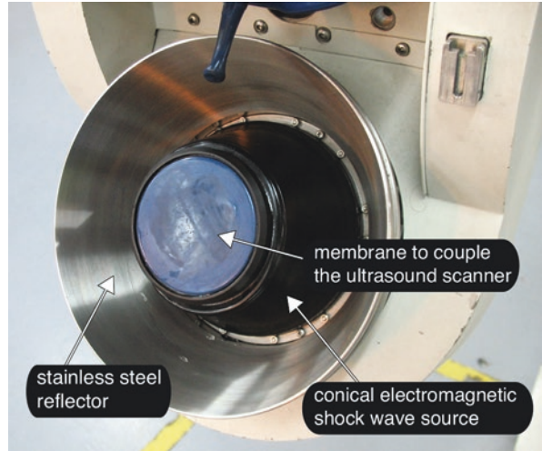
Fig. 5.50 Photograph of one of the two conical coil shock wave generators of a Duet Magna lithotripter without the latex membrane that covers the shock wave source. (Courtesy of Direx Systems Corporation, Canton MA, USA)
