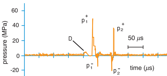
Fig. 5.35 Pressure waveform recorded with a PVDF needle hydrophone at the F2 focus of a dual-phase reflector, showing the arrival of the direct, non-reflected shock wave (D), followed by a standard lithotripter shock wave and a phase-inverted pressure waveform
