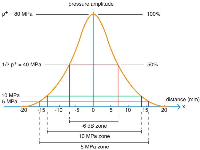
Fig. 3.9 The pressure as a function of the distance along an axis perpendicular to the beam axis of a shock wave source, showing the difference in size between the -6 dB, 10 MPa and 5 MPa focal zones. The peak-positive pressure p^+ of 80 MPa was arbitrarily selected as an example
