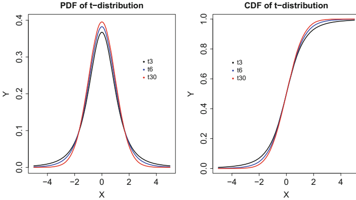
Fig. 4.8 pdf (left) and cdf (right) of t -distribution with different degrees of freedom (t3 stands for t -distribution with degree of freedom 3) MVAtdis
