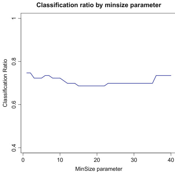
Fig. 20.32 Successful classification ratio dynamic over the number of terminal nodes: cross-validation MVAbancrupcydis
