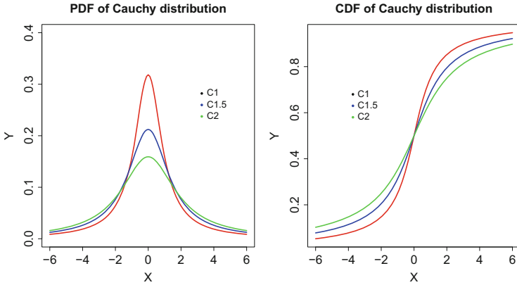
Fig. 4.11 pdf (left) and cdf (right) of Cauchy distribution with m = 0 and different scale parameters (C1 stands for Cauchy distribution with s = 1 ) MVAcachy
