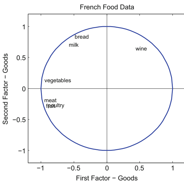
Fig. 11.8 Representation of the variables MVA n pca food
