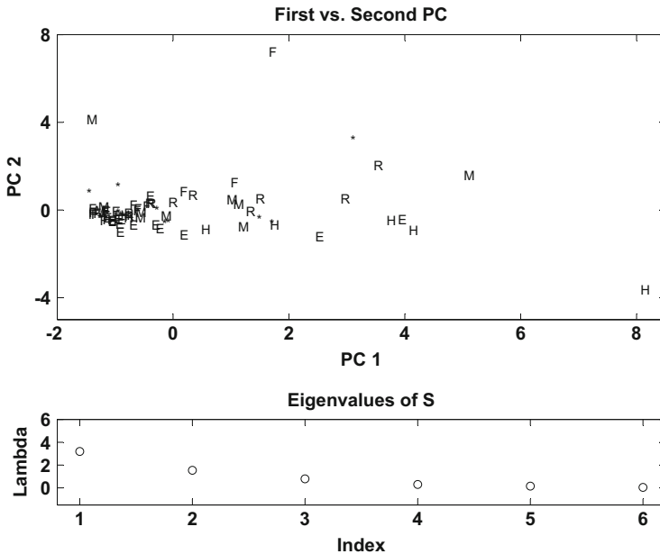
Fig. 11.16 Principal components of the US company data (without IBM and General Electric) MVAnpcausco2
