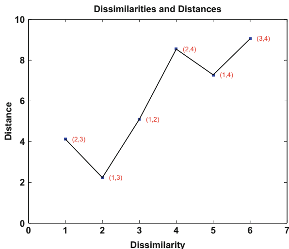
Fig. 17.8 Scatterplot of dissimilarities against distances MVAAnmds2
