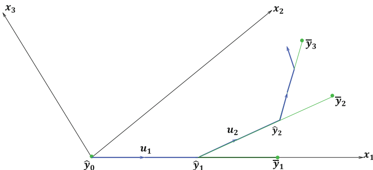
Fig. 9.2 Illustration of LARS algorithm
