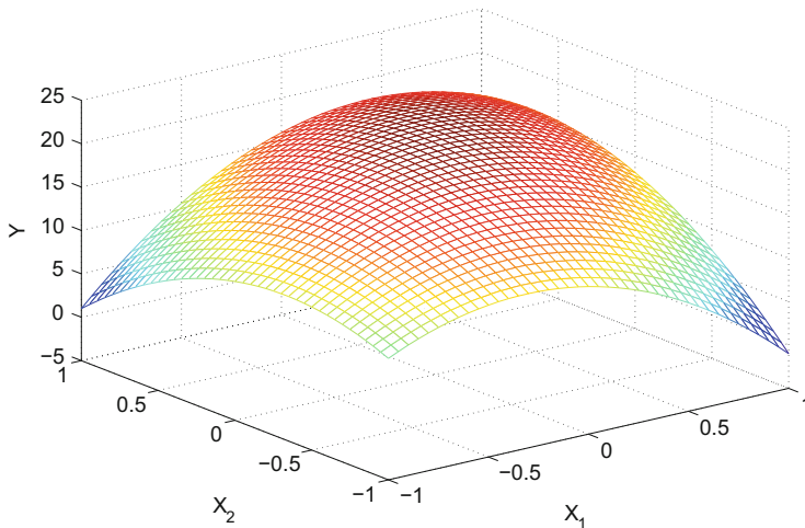
Fig. 8.1 A 3-D response surface MVAresponsesurface
