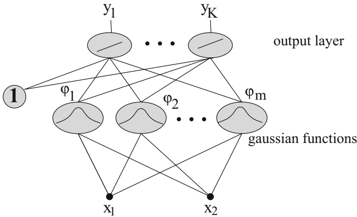
Fig. 5.6 Radial-basis function network
