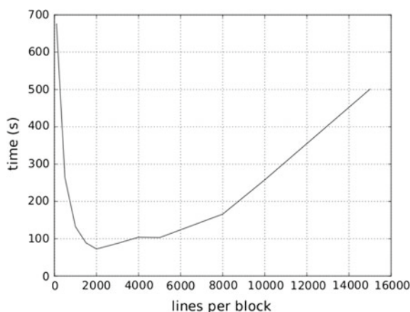
Fig. 11.3 Performance to process 1 million lines of a CSV file using 8 engines for different values of lines per block. Time is shown in seconds
