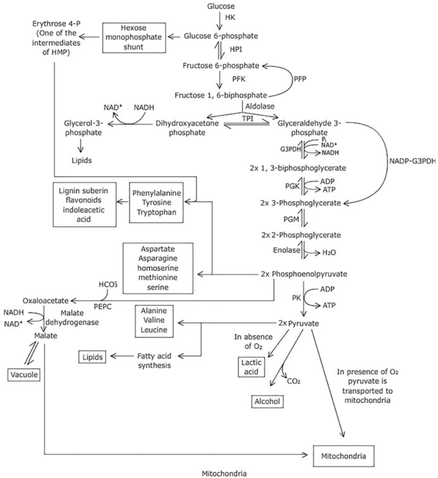
Fig. 7.3 Cytosolic glycolytic pathway and its role in metabolism of plants. HK, hexokinase; HPI, hexose phosphate isomerase; PFK, phosphofruktokinase; G3PDH, glyceraldehyde 3-phosphate dehydrogenase; PGK, phosphoglycerate kinase; PGM, phosphoglyceromutase; PK, pyruvate kinase; PEPC, PEP carboxylase; TPI, triose phosphate isomerase; HMP, hexose monophosphate pathway
