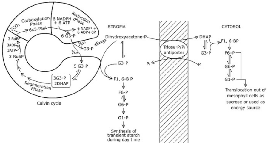
Fig. 5.17 Triose P/P i antiporter localized on the inner membrane of plastid facilitates the exchange of triose-P between stroma of the plastid and cytosol
