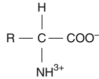
\alpha - Amino acid
