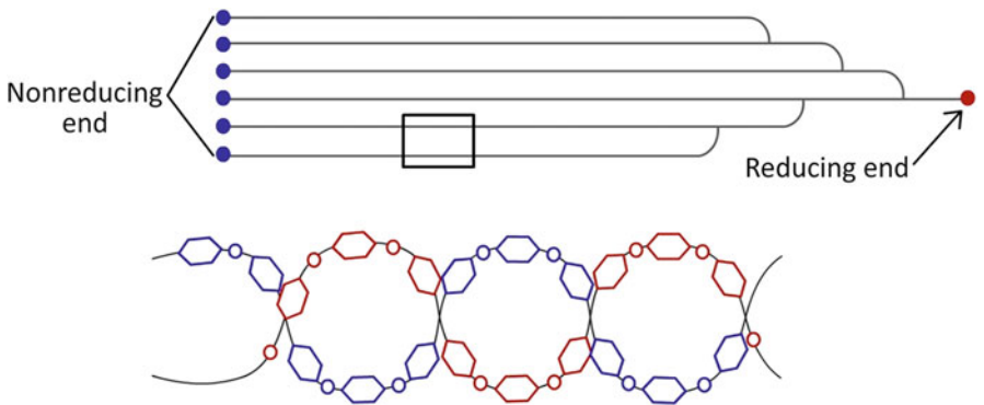
Fig. 9.15 In amylopectin, α-D glucosyl residues are joined by α-(1-4)-glycosidic bonds similar to those in amylose. However, unlike amylose, amylopectin is a highly branched polymer because of the presence of α-(1-6)-glycosidic linkages after every 20–26 glucosyl residues. Hydrogen bonds are formed in between hydroxyl groups of adjacent chains as a result of which double helical structure is formed in amylopectin either in between adjacent branches of the molecule itself or with amylose polymer
