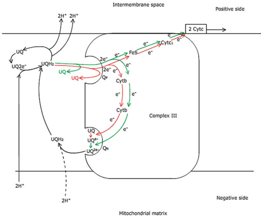
Fig. 7.24 Q-cycle. In the first cycle, out of the two electrons removed from \text{UQH}_2 , one electron is transferred to \text{cyt c} , and one is cycle back to \text{UQ} via \text{cyt b} (demonstrated in red). Similar cycle is repeated from another molecule of \text{UQH}_2 (demonstrated in green). This results in reduction of \text{UQ}^{e^-} to \text{UQ}^{2e^-} .
