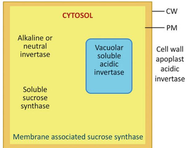
Fig. 9.12 Several isoforms of invertase and sucrose synthase: Invertase found in apoplast (cell wall) and vacuoles has acidic pH optima (5.0), while cytosolic invertase has alkaline pH optima (7.5). Sucrose synthase is present as soluble form in cytosol or is associated with plasma membrane in insoluble form
