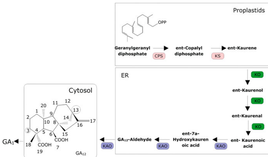
Fig. 17.2 Gibberellin biosynthesis. CPS ent -copalyl diphosphate synthase, KS ent -kaurene synthase, KO ent -kaurene oxidase, KAO ent -kaurenoic acid oxidase; encircled carbon atoms on GA 12 are oxidized for the synthesis of GA 1
