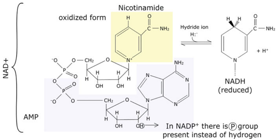
Fig. 4.9 Reduction of \text{NAD}^+ to \text{NADH} requires two-electron transfer. Only nicotinamide ring is affected. Hydride ion (a proton with two electrons) transfer results in reduction of \text{NAD}^+ to \text{NADH} . \text{NADP}^+ differs from \text{NAD}^+ only in presence of phosphoryl group on the 2'-hydroxyl group of ribose sugar. Plus (+) sign on \text{NAD}^+ and \text{NADP}^+ indicates that nicotinamide ring is in oxidized form and there is positive charge on the nitrogen atom of the ring. In many cells ratio of \text{NAD}^+ to \text{NADH} is high which favors hydride transfer to \text{NAD}^+ to form \text{NADH} . Contrary to this ratio of \text{NADPH} to \text{NADP}^+ is high which favors hydride transfer from \text{NADPH} to substrates. In most of the cells, total concentration of \text{NAD}^+ + \text{NADH} is about 10^{-5} M, while that of \text{NADPH} + \text{NADP}^+ is 10^{-6} M
