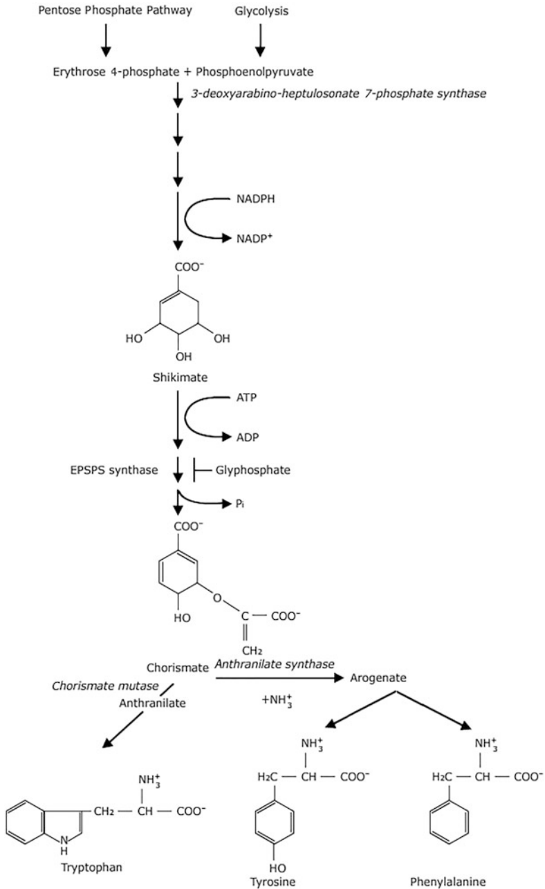
Fig. 33.8 Shikimic acid pathway for biosynthesis of phenolics
