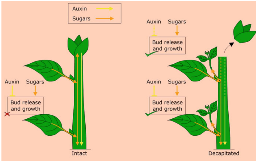
Fig. 15.12 Regulation of apical dominance by sugar availability
