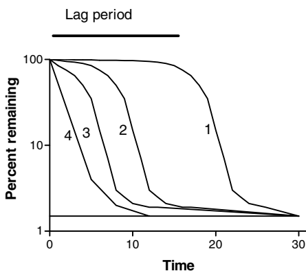
Figure 8.5 Disappearance of a substance when there is an adaption phase (1) with a long lag period, for instance, when MCPA or another herbicide that can support some microorganisms is applied for the first time. After having been used for several years, the degradation starts almost immediately (2 and 3). A small residual amount (e.g., 1.5%) is not degraded, due to strong binding to the soil or because the concentration is too low to be of interest to the microorganisms. Co-metabolism or complete adaption is shown by (4).
