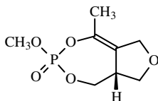
The acetylcholinesterase inhibitor from S. antibioticus
