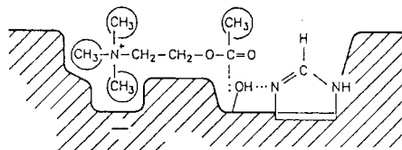
Figure 5.3 The classical model of the active site of acetylcholinesterase.
