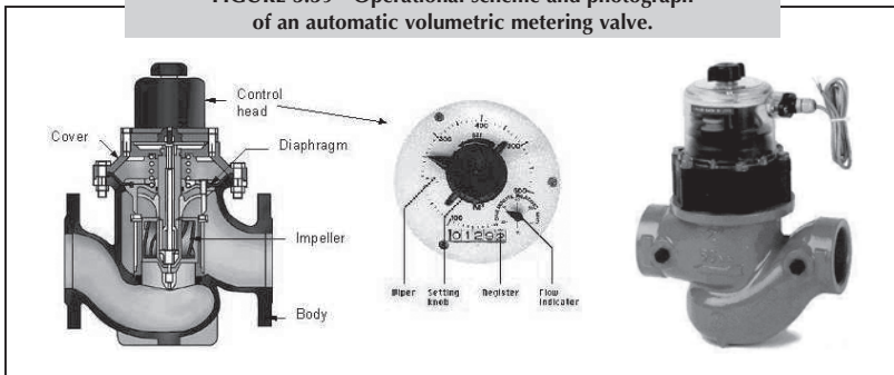
FIGURE 3.39 - Operational scheme and photograph of an automatic volumetric metering valve.
