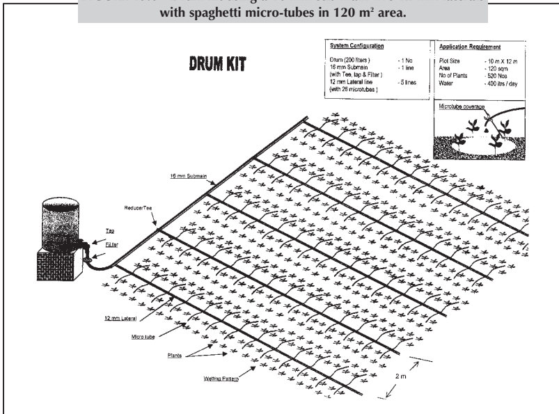
FIGURE 15.6 - Drum kit using a 16 mm sub-main five 12 mm laterals with spaghetti micro-tubes in 120 m 2 area.
