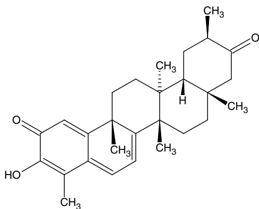
FIGURE 9.40 Tingenone.
