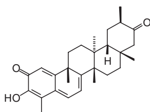
tingenone
