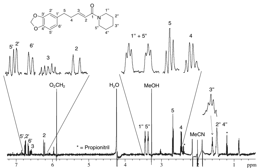
FIGURE 9.93 Dihydropiperlonguminine.
