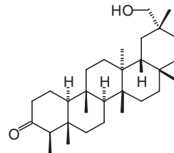
29-hydroxyfriedelan-3-one
