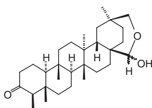
30-hydroxyfriedelan-3-on-28-al hemiacetals
