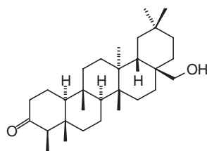
canophyllol
