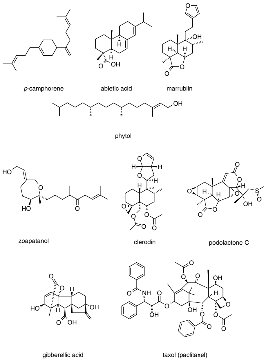
FIGURE 1.14 Assorted diterpenes.
