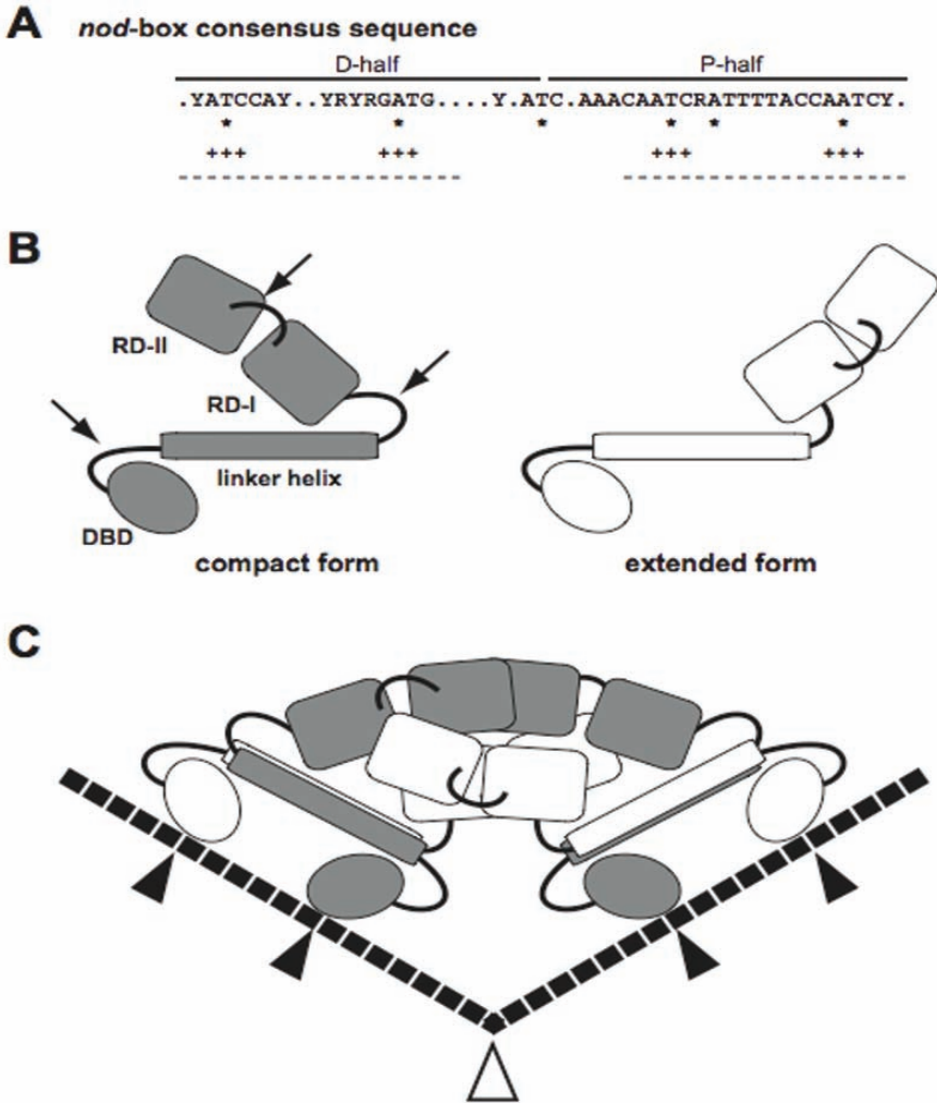
Figure 1. Interaction between LysR type transcriptional regulator (LTTR) and the target promoter.
