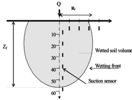
FIGURE 4.1 Schematic description of the wetted cross-section and the location of sensors to measure soil water suction at the experimental site (Fig. 4.2). R_f = Radius of the wetted surface, Z_f = Depth of the wetted bulb, and Q = Discharge rate from the emitter.
