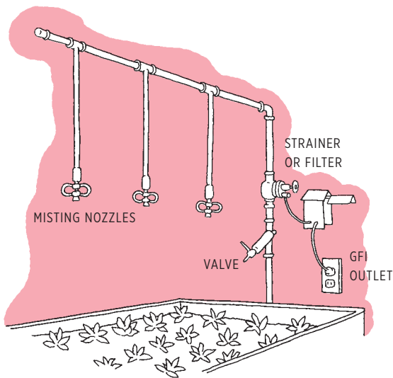
An overhead misting system feeds water through a filter out of misting nozzles.
