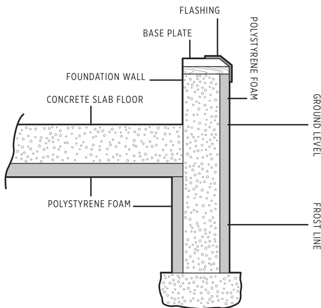
Insulate a concrete foundation.
