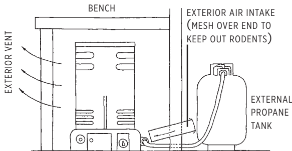
A portable heater can be fueled by an external propane tank.
