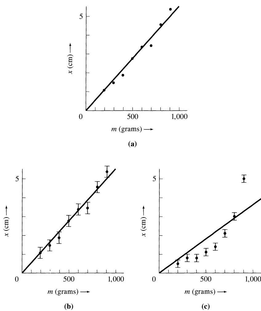
Figure 2.5. Three plots of extension x of a spring against the load m . (a) The data of Table 2.3 without error bars. (b) The same data with error bars to show the uncertainties in x . (The uncertainties in m are assumed to be negligible.) These data are consistent with the expected proportionality of x and m . (c) A different set of data, which are inconsistent with x being proportional to m .
