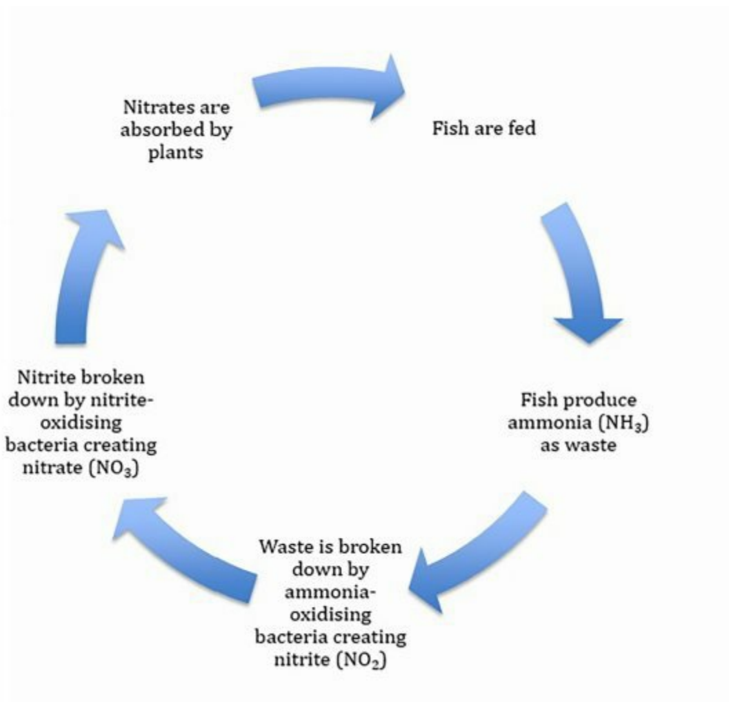
Figure 3: The nitrogen cycle in an aquaponics system
