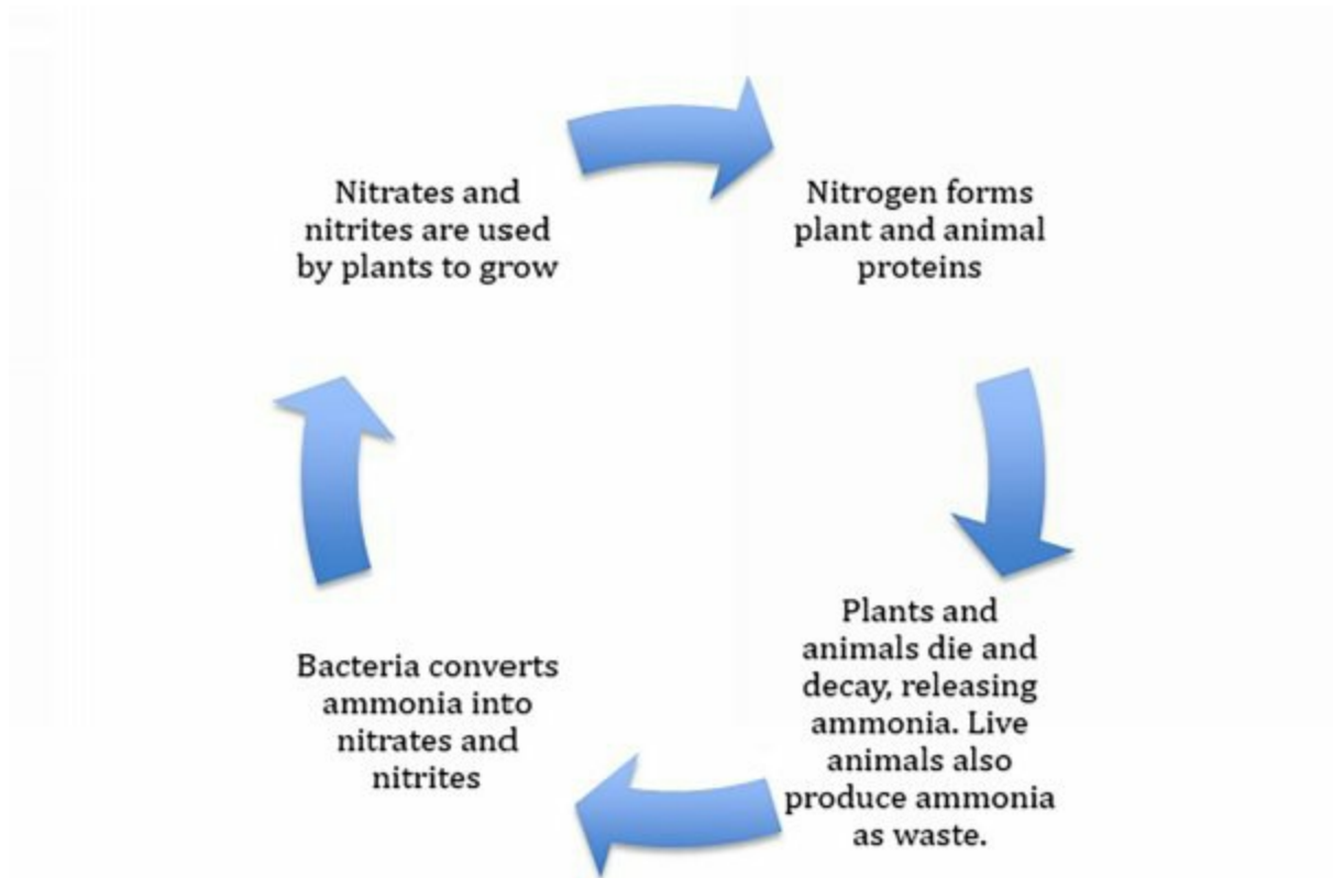
Figure 2: The nitrogen cycle
