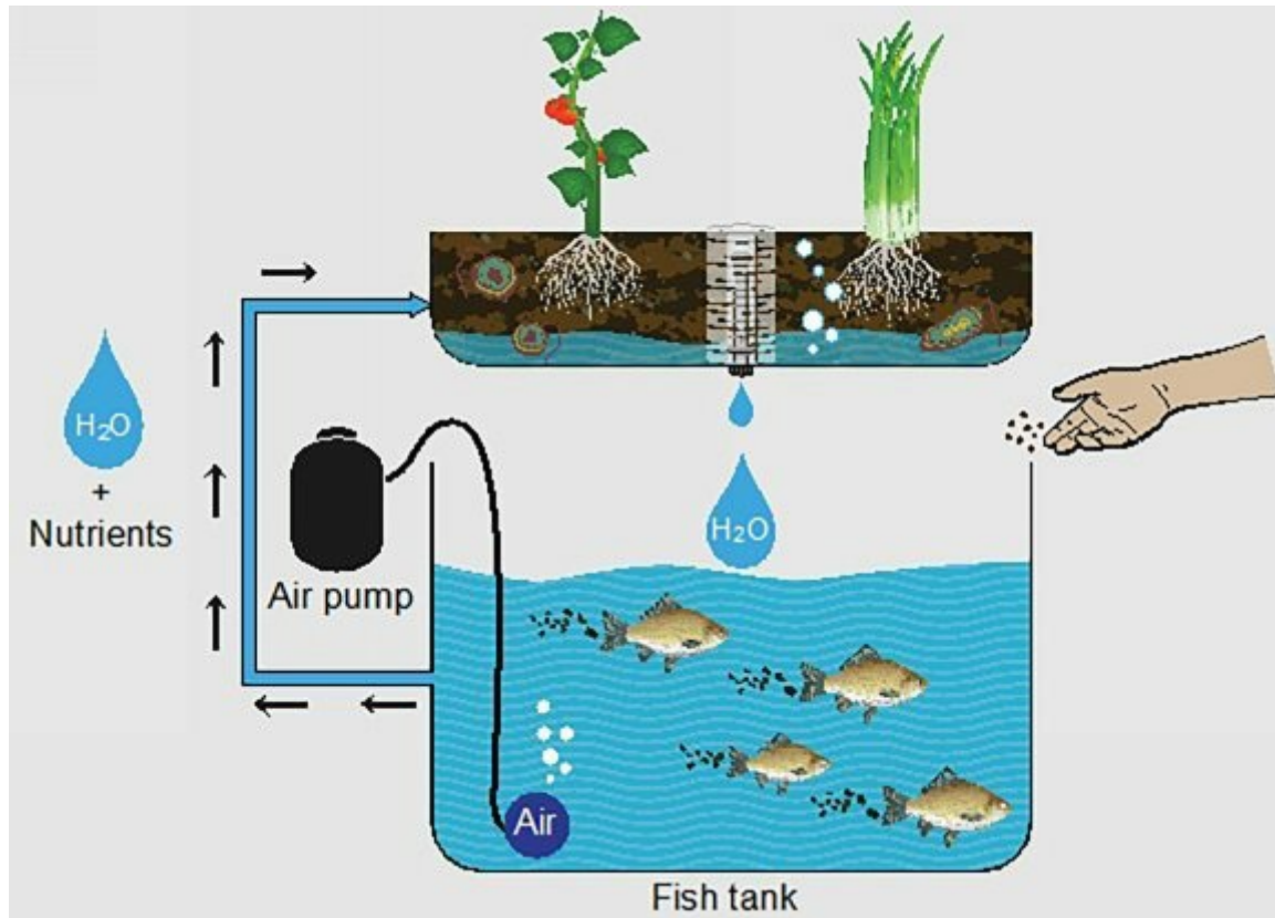
Figure 4: Basic aquaponic unit
