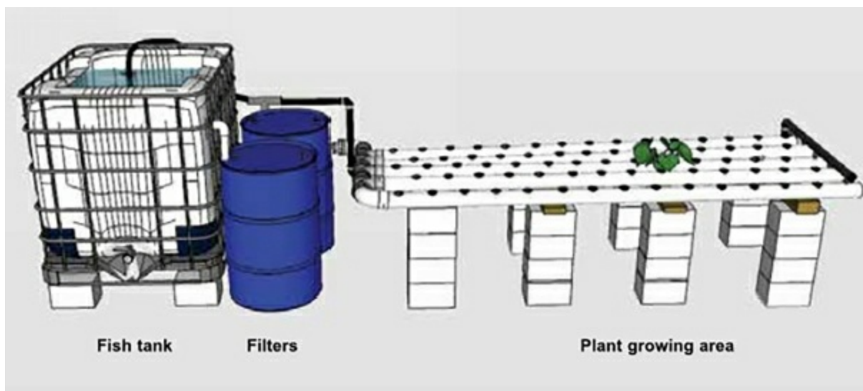
Figure 6: NFT Unit
