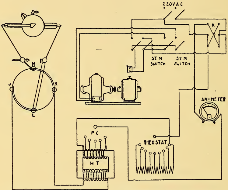
FIG. 20.—Diagram of connections of an "interrupterless" apparatus operating on an alternating current.
