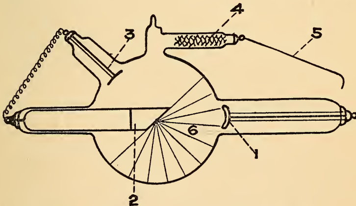
FIG. 9.—Modern type of Röntgen-ray or focus tube. 1, cathode; 2, target; 3, accessory anode; 4, vacuum regulator; 5, adjustable wire; 6, X-ray hemisphere.
