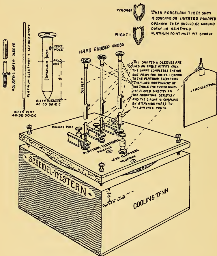
FIG. 14.—The Wehnelt electrolytic interrupter.
