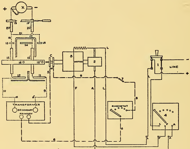
Fig. 17.—Diagram of connections of interrupterless apparatus.
