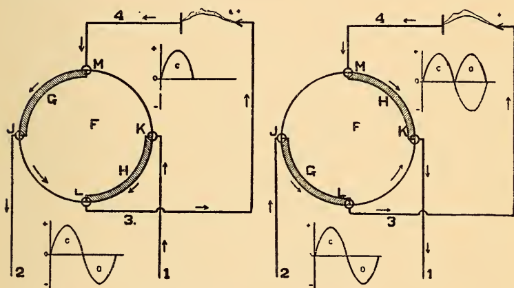
Figs. 18 and 19.—Illustrating rectification of current by revolving discs.
