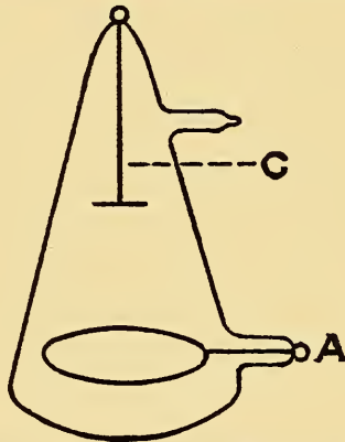
FIG. 7.—Early type of Röntgen-ray tube.
