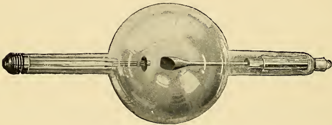
FIG. 11.—The Coolidge tube.
