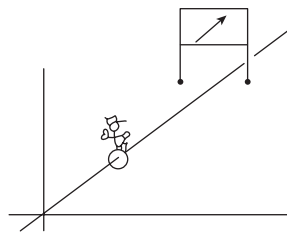
Figure 13.6 The photon pilot
