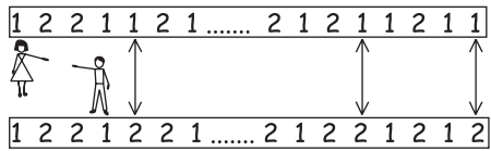
Figure 13.5 Experiment IV: Both Alice's and Bob's polarizers are rotated, and mismatches are due to both rotations
