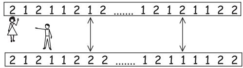
Figure 13.4 Experiment II: Alice's polarizer is rotated, causing mismatches
