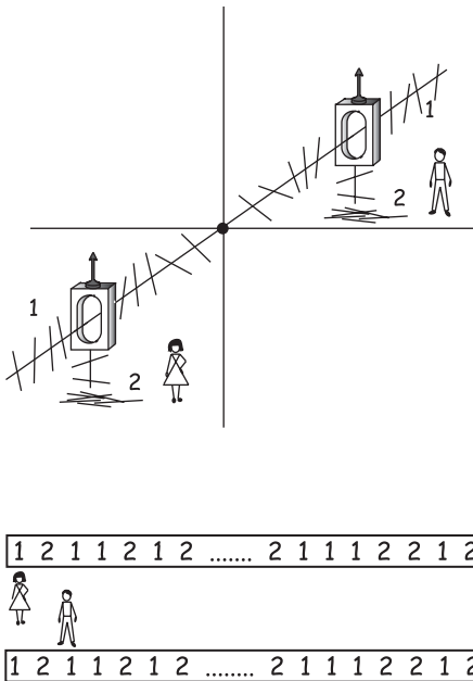
Figure 13.3 Experiment I: Polarizers are aligned, and Alice’s and Bob’s data are identical
