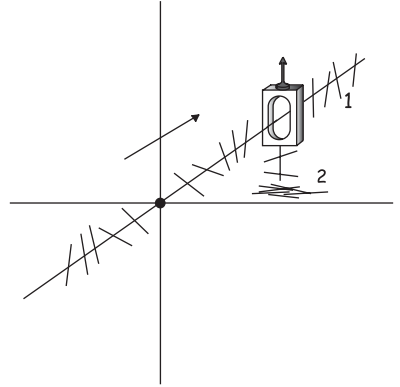
Figure 13.2 Model of stick photons and oval polarizer
