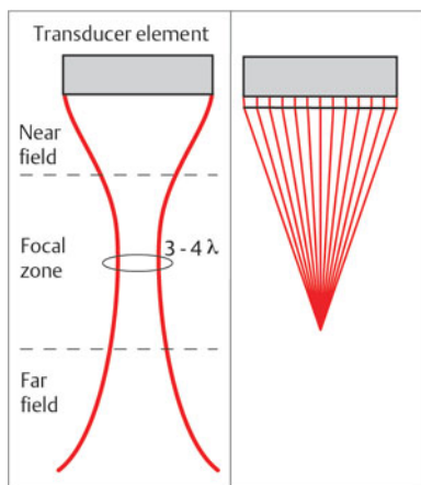
Fig. 1 Ultrasound beam shape and electronic focusing (after R othlin, Bouillon, and Klotter)
