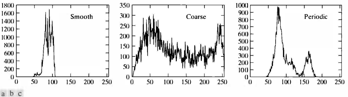
FIGURE 12.22 Histograms corresponding to the subimages in Fig. 12.21.
