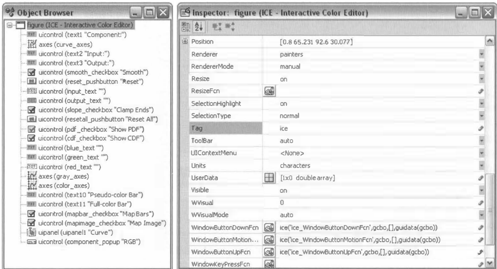
FIGURE B.2 The (a) GUIDE Object Browser and (b) Property Inspector for the ICE “figure” object.
