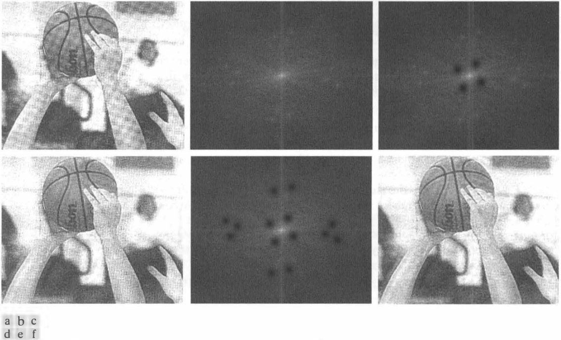
FIGURE 4.21 (a) Scanned, 72 dpi newspaper image of size 232 \times 288 pixels corrupted by a moiré pattern. (b) Spectrum. (c) Gaussian notch filters applied to the low-frequency bursts caused by the moiré pattern. (d) Filtered result. (e) Using more filters to eliminate higher frequency “structured” noise. (f) Filtered result.
