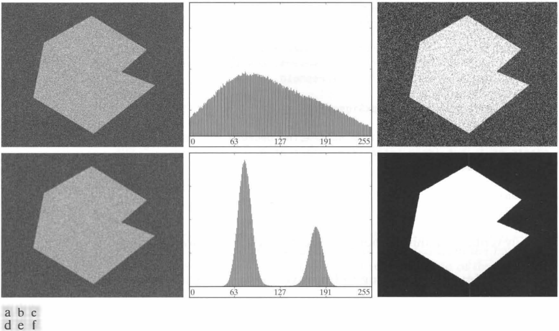
FIGURE 11.15 (a) Noisy image, and (b) its histogram. (c) Result obtained using Otsu's method. (d) Noisy image smoothed using a 5 \times 5 averaging mask, and (e) its histogram. (f) Result of thresholding using Otsu's method.
