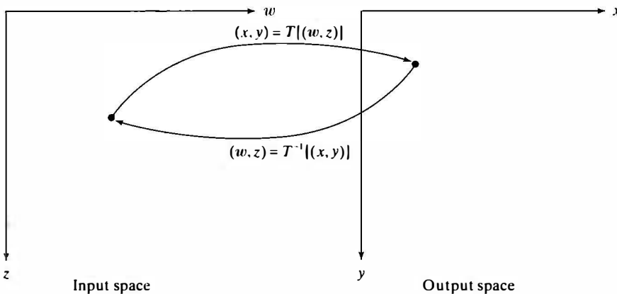
FIGURE 6.1 Forward and inverse transformation of a point for T[(w, z)] = (w/2, z/2) .
