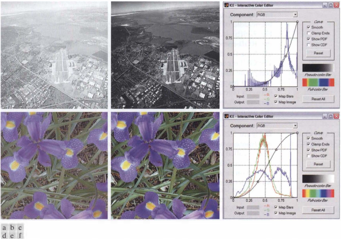
FIGURE 7.18 Using function ice for monochrome and full color contrast enhancement: (a) and (d) are the input images, both of which have a “washed-out” appearance; (b) and (e) show the processed results; (c) and (f) are the ice displays. (Original monochrome image for this example courtesy of NASA.)
