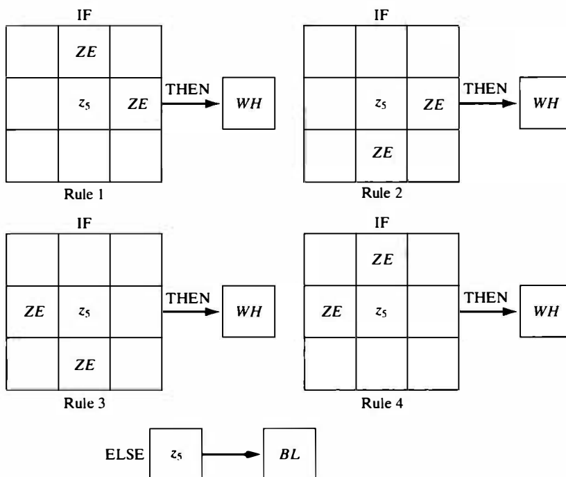
FIGURE 3.32 Fuzzy rules for boundary detection.
