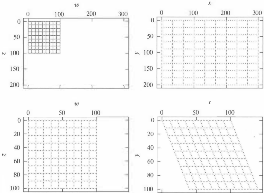
FIGURE 6.3 Visualizing the effect of spatial transformations on a grid of points. (a) Grid 1. (b) Grid 1 transformed using tform1. (c) Grid 2. (d) Grid 2 transformed using tform2.
