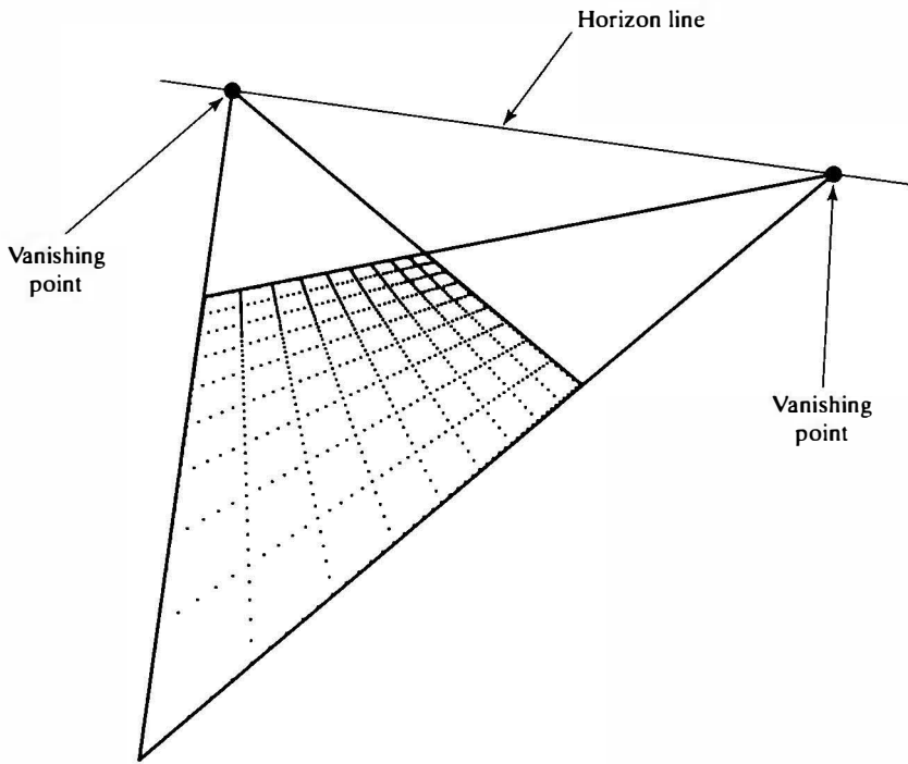
FIGURE 6.6 Vanishing points and the horizon line for a projective transformation.
