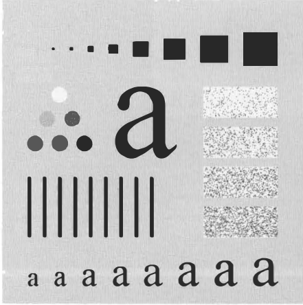
FIGURE 8.8 Wavelet-based image smoothing: (a) A test image; (b) its wavelet transform; (c) the inverse transform after zeroing the first level detail coefficients; and (d) through (f) similar results after zeroing the second-, third-, and fourth-level details.
