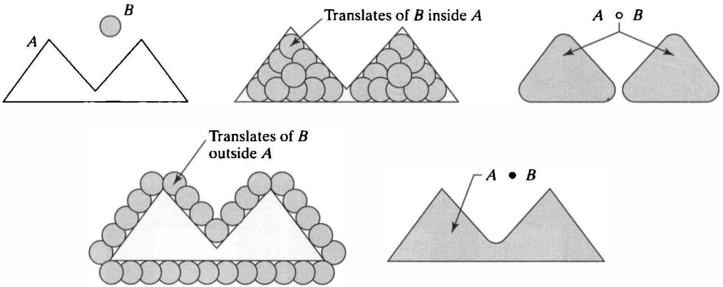
FIGURE 10.9 Opening and closing as unions of translated structuring elements. (a) Set A and structuring element B . (b) Translations of B that fit entirely within set A . (c) The complete opening (shaded). (d) Translations of B outside the border of A . (e) The complete closing (shaded).
