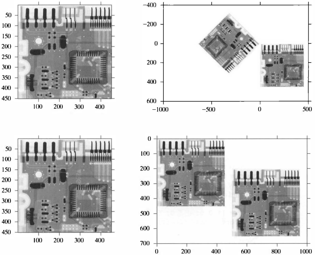
FIGURE 6.11 (a) Original image. (b) Original and rotated image displayed using common coordinate system. (c) Translated image as computed using basic imtransform syntax. (d) Original and translated image displayed using common coordinate system.
