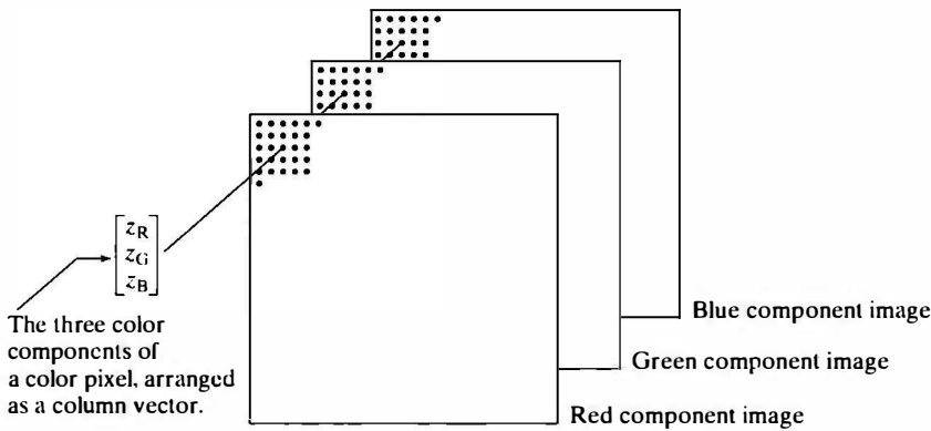
FIGURE 7.1 Schematic showing how pixels of an RGB color image are formed from the corresponding pixels of the three component images.
