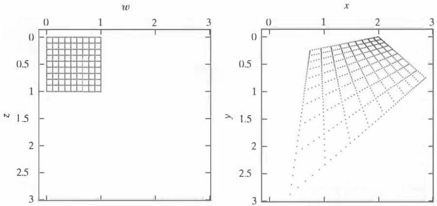
a b FIGURE 6.5 Example of a projective transformation. (a) Point grid in input space. (b) Transformed point grid in output space.
