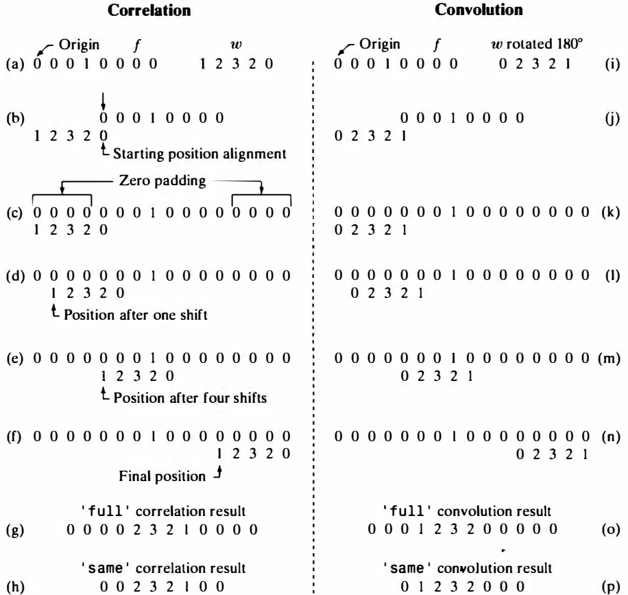
FIGURE 3.14 Illustration of one-dimensional correlation and convolution.
