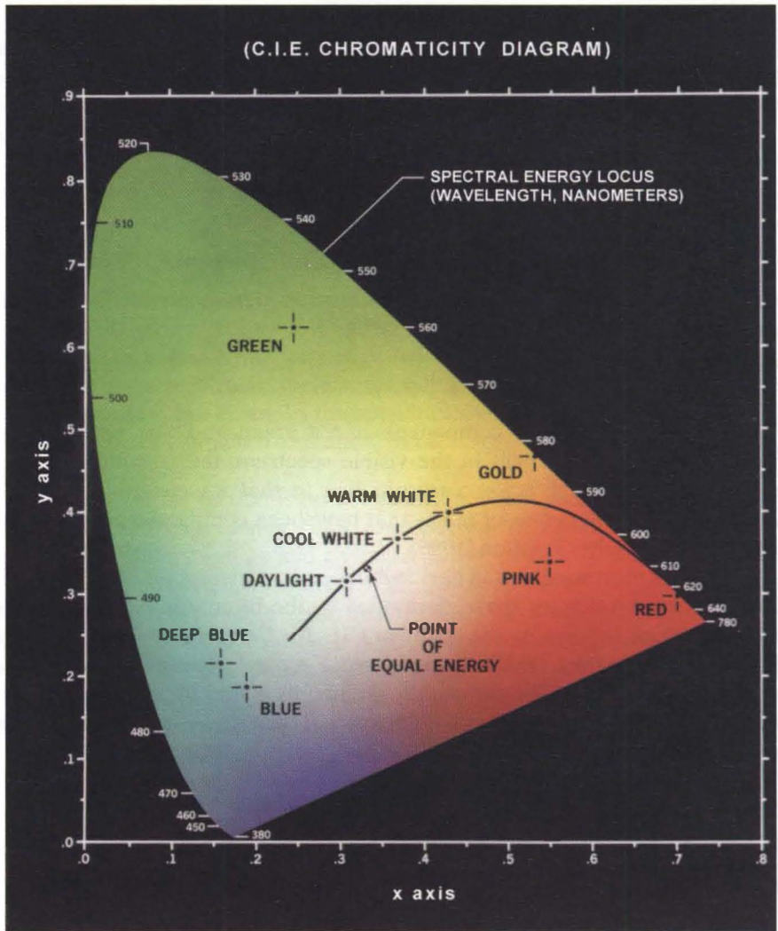
FIGURE 7.10 CIE chromaticity diagram. (Courtesy of the General Electric Co. Lamp Business Division.)
