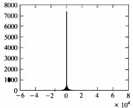
FIGURE 9.19 (a) The second frame of a 16-frame video of the space shuttle in orbit around the Earth. The first and last frames are shown in Fig. 9.18. (b) The histogram of the prediction error resulting from the previous frame prediction in Example 9.9. (Original image courtesy of NASA).
