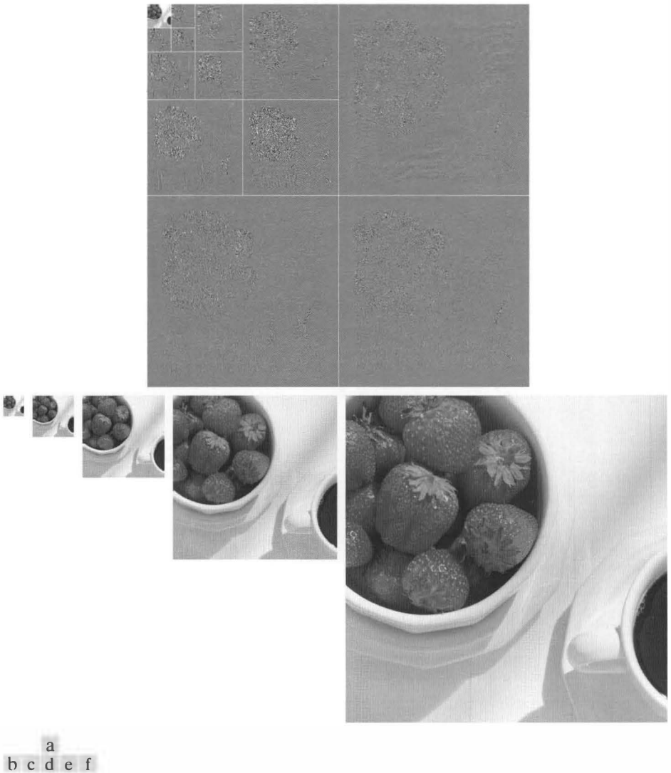
FIGURE 8.9 Progressive reconstruction: (a) A four-scale wavelet transform; (b) the fourth-level approximation image from the upper-left corner; (c) a refined approximation incorporating the fourth-level details; (d) through (f) further resolution improvements incorporating higher-level details.
