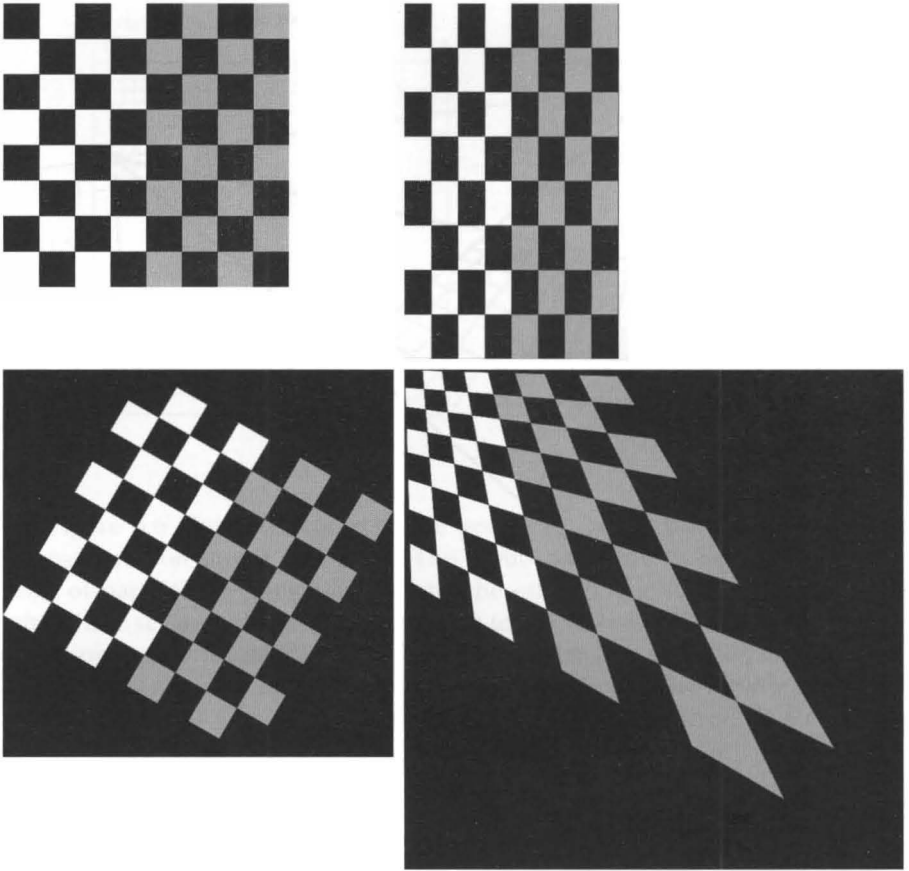
FIGURE 6.7 Geometric transformations of the checkerboard image.
