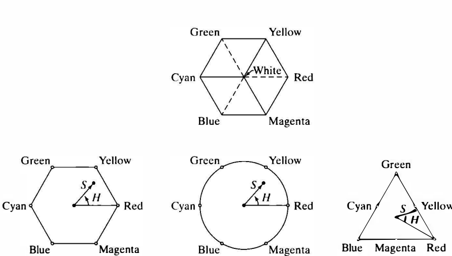
FIGURE 7.7 Hue and saturation in the HSI color model. The dot is an arbitrary color point. The angle from the red axis gives the hue, and the length of the vector is the saturation. The intensity of all colors in any of these planes is given by the position of the plane on the vertical intensity axis.
