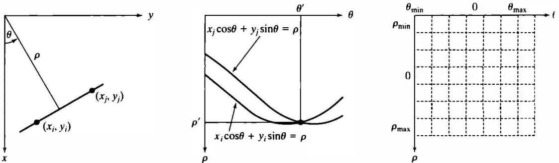
FIGURE 11.9 (a) Parameterization of lines in the xy -plane. (b) Sinusoidal curves in the \rho\theta -plane; the point of intersection, (\rho', \theta') , corresponds to the parameters of the line joining (x_i, y_i) and (x_j, y_j) . (c) Division of the \rho\theta -plane into accumulator cells.
