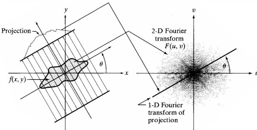
FIGURE 5.15 Graphical illustration of the Fourier slice theorem.
