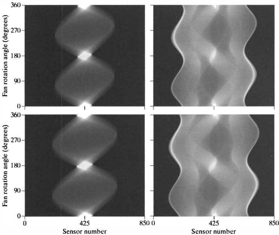
a b c d FIGURE 5.23 Illustration of function fanbeam. (a) and (b) Linear fan-beam projections for the rectangle and phantom images generated with function fanbeam. (c) and (d) Corresponding arc projections.
