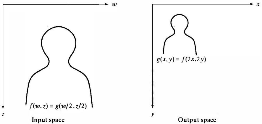
FIGURE 6.2 Forward and inverse transformation of a simple image for the transformation T[(w, z)] = (w/2, z/2) .
