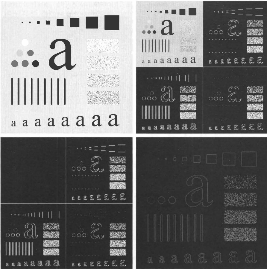
FIGURE 8.7 Wavelets in edge detection: (a) A simple test image; (b) its wavelet transform; (c) the transform modified by zeroing all approximation coefficients; and (d) the edge image resulting from computing the absolute value of the inverse transform.
