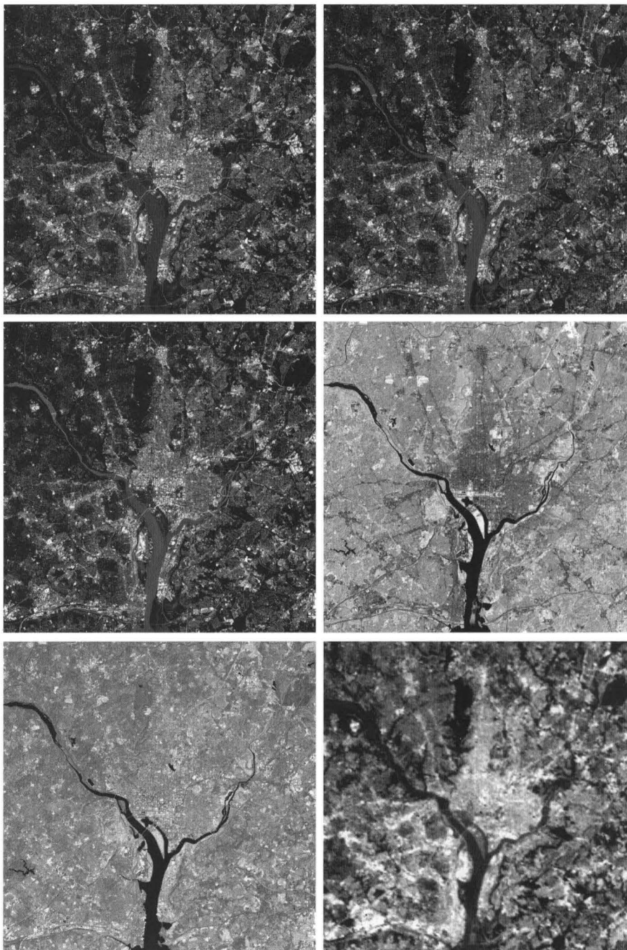
FIGURE 12.30 Six multispectral images in the (a) visible blue, (b) visible green, (c) visible red, (d) near infrared, (e) middle infrared, and (f) thermal infrared bands. (Images courtesy of NASA.)
