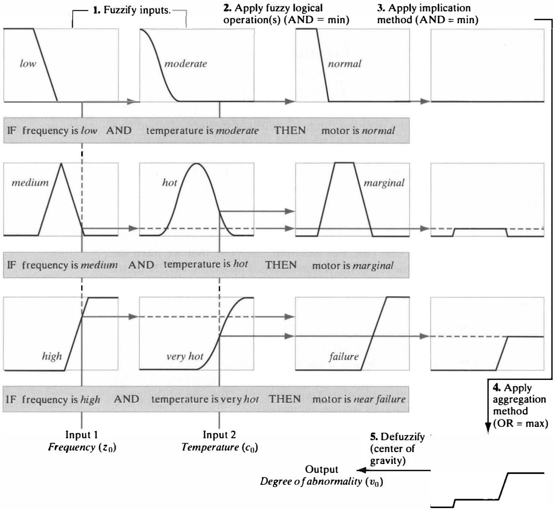
FIGURE 3.25 Example illustrating the five basic steps used typically to implement a fuzzy rule-based system: (1) fuzzification, (2) logical operations, (3) implication, (4) aggregation, and (5) defuzzification.
