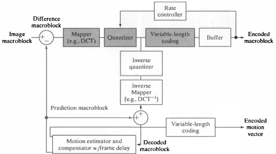
FIGURE 9.21 A typical motion compensated video encoder.
