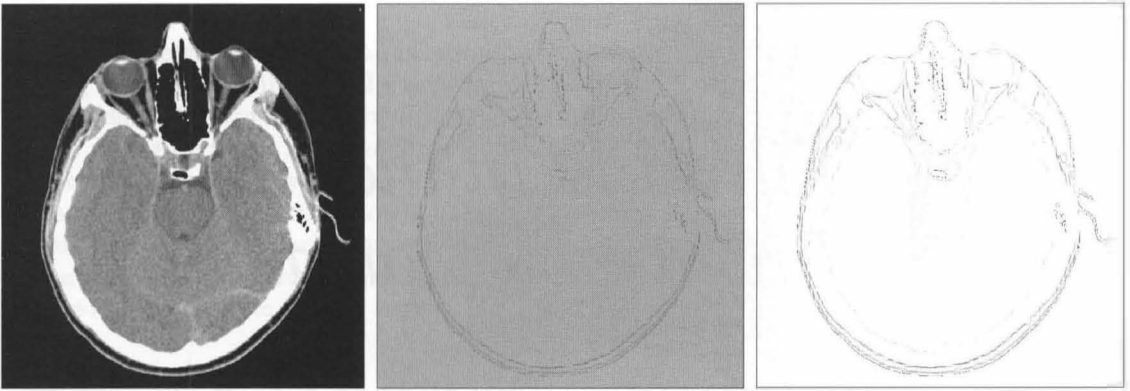
FIGURE 3.33 (a) CT scan of a human head. (b) Result of fuzzy spatial filtering using the membership functions in Fig. 3.31 and the rules in Fig. 3.32. (c) Result after intensity scaling. The thin black picture borders in (b) and (c) were added for clarity; they are not part of the data. (Original image courtesy of Dr. David R. Pickens, Vanderbilt University.)
