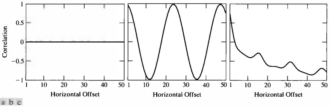
FIGURE 12.25 Values of the correlation descriptor as a function of horizontal offset (distance between adjacent pixels) corresponding to (a) the noisy, (b) the sinusoidal, and (c) the circuit board images in Fig. 12.24.
