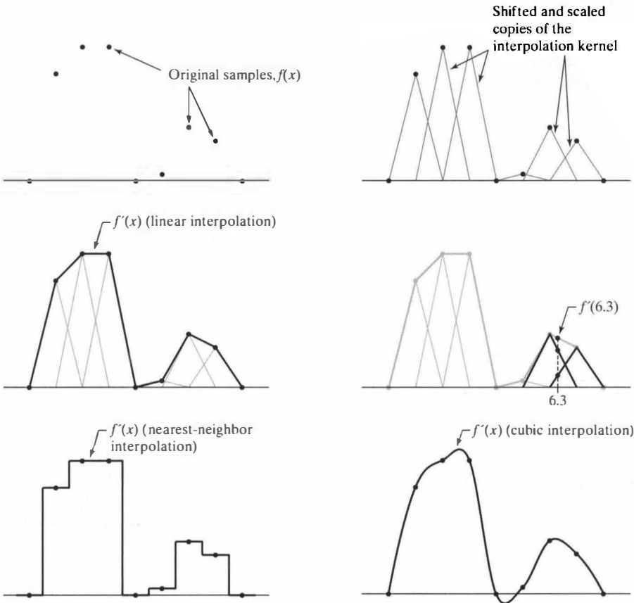
FIGURE 6.15 (a) Original samples, f(x) . (b) Copies of triangular interpolation kernel, h_T(x) , shifted and then scaled by the values of f(x) . (c) Sum of the shifted and scaled interpolation kernels, resulting in f'(x) as computed using linear interpolation. (d) Computing f'(6.3) as f(6)h_T(0.3) + f(7)h_T(0.7) . (e) f'(x) computed using nearest-neighbor interpolation. (f) f'(x) computed using cubic interpolation.
