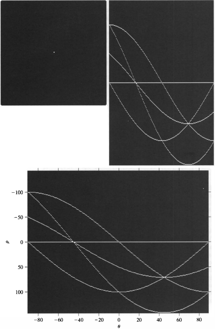
FIGURE 11.10 (a) Binary image with five dots (four of the dots are in the corners). (b) Hough transform displayed using imshow . (c) Alternative Hough transform display with axis labeling. [The dots in (a) were enlarged to make them easier to see.]
