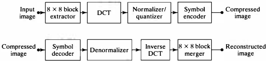
FIGURE 9.11 JPEG block diagram: (a) encoder and (b) decoder.
