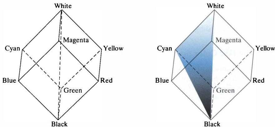
FIGURE 7.6 Relationship between the RGB and HSI color models.
