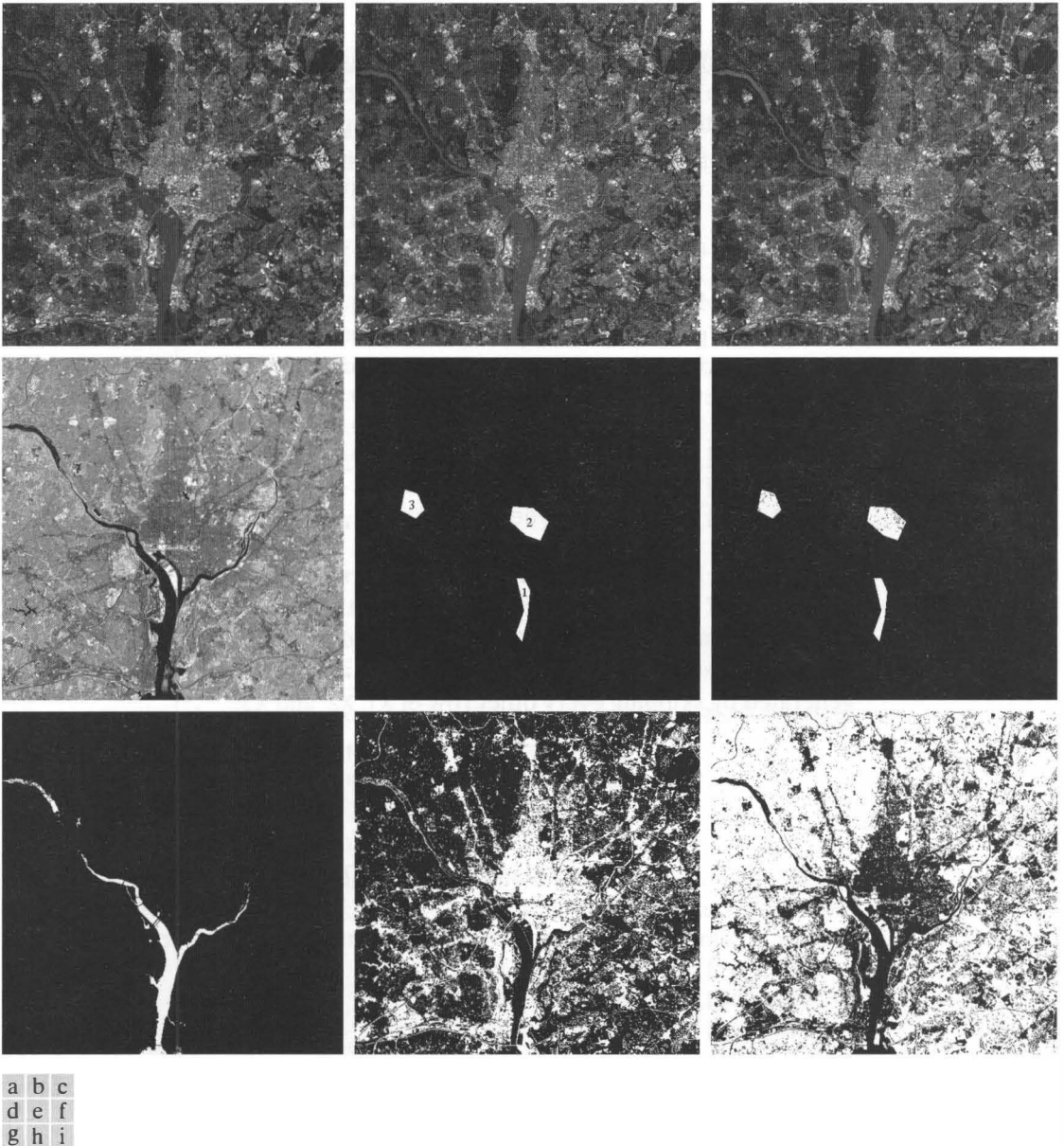
FIGURE 13.2 Bayes classification of multispectral data. (a)-(d) Images in the visible blue, visible green, visible red, and near infrared wavelengths. (e) Masks showing sample regions of (1) water, (2) urban development, and (3) vegetation. (f) Results of classification; the black dots denote points classified incorrectly. The other (white) points were classified correctly. (g) All image pixels classified as water (in white). (h) All image pixels classified as urban development (in white). (i) All image pixels classified as vegetations (in white). All images are of size 512 \times 512 pixels.
