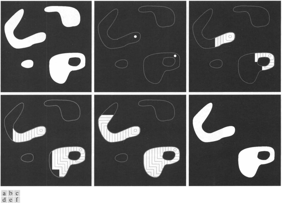
FIGURE 10.21 Morphological reconstruction. (a) Original image (the mask). (b) Marker image. (c)–(e) Intermediate result after 100, 200, and 300 iterations, respectively. (f) Final result. (The outlines of the objects in the mask image are superimposed on (b)–(e) as visual references.)
