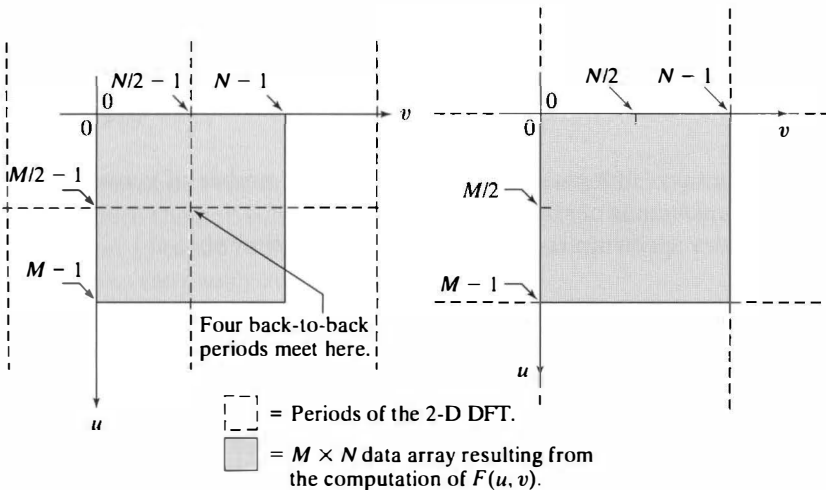
FIGURE 4.2 (a) M \times N Fourier spectrum (shaded), showing four back-to-back quarter periods. (b) Spectrum after multiplying f(x, y) by (-1)^{x+y} prior to computing the Fourier transform. The shaded period is the data that would be obtained by using the DFT.
