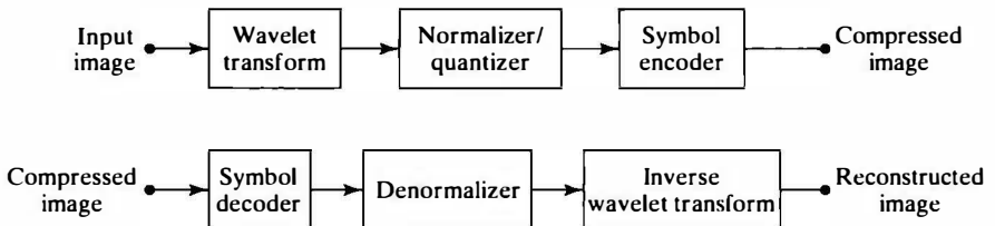
FIGURE 9.14 JPEG 2000 block diagram: (a) encoder and (b) decoder.
