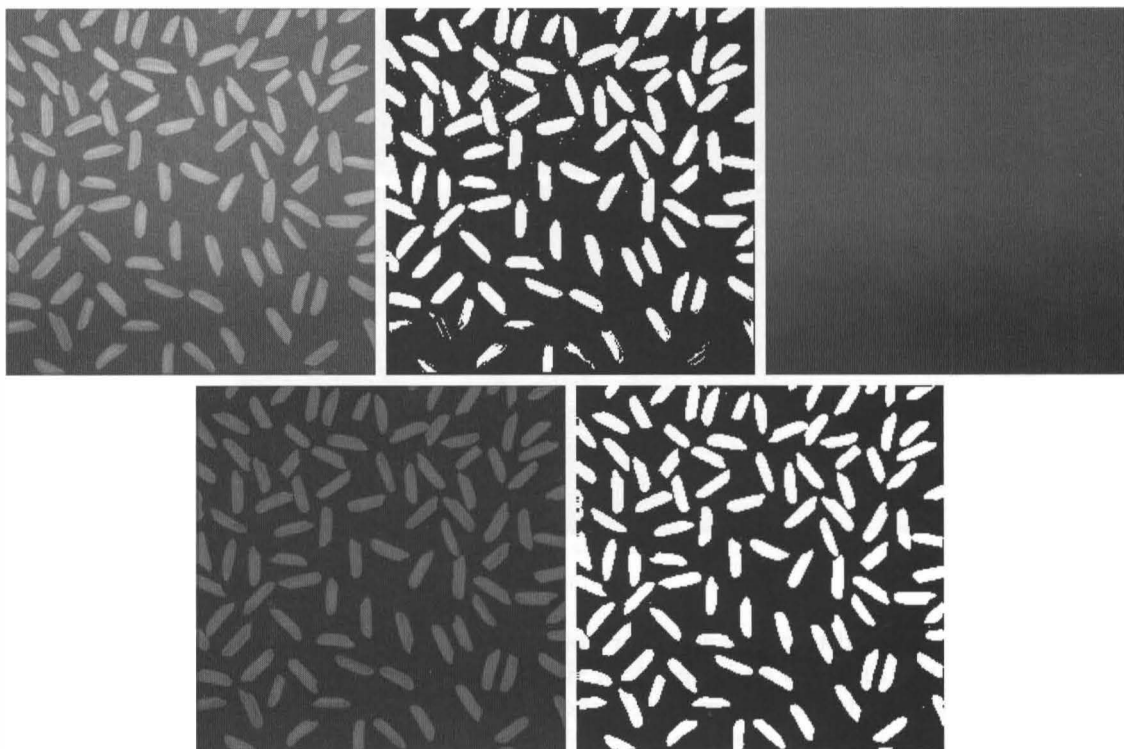
FIGURE 10.26 Compensating for non-uniform illumination. (a) Original image. (b) Thresholded image. (c) Opened image showing an estimate of the background. (d) Result of subtracting the estimated background for the original image. (e) Result of thresholding the image in (d). (Original image courtesy of The MathWorks, Inc.)
