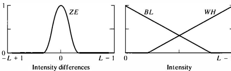
FIGURE 3.31 Membership function of the fuzzy set zero ( ZE ). (b) Membership functions of the fuzzy sets black ( BL ) and white ( WH ).
