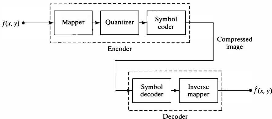
FIGURE 9.1 A general image compression system block diagram.
