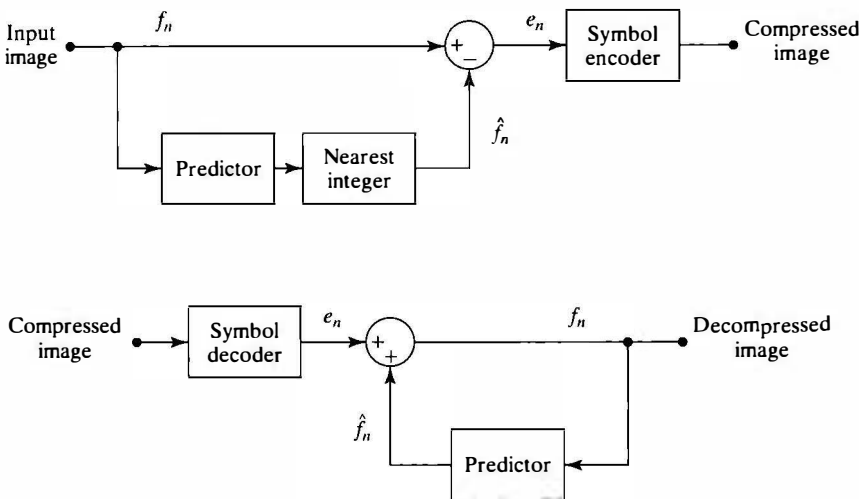
FIGURE 9.8 A lossless predictive coding model: (a) encoder and (b) decoder.
