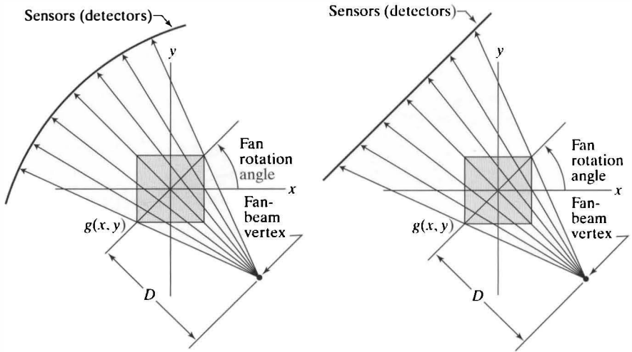
a b FIGURE 5.22 The arc and linear fan-beam projection capabilities of function fanbeam. g(x, y) refers to the image region shown in gray.
