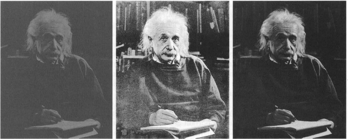
FIGURE 3.28 (a) Low-contrast image. (b) Result of histogram equalization. (c) Result of fuzzy, rule-based, contrast enhancement.
