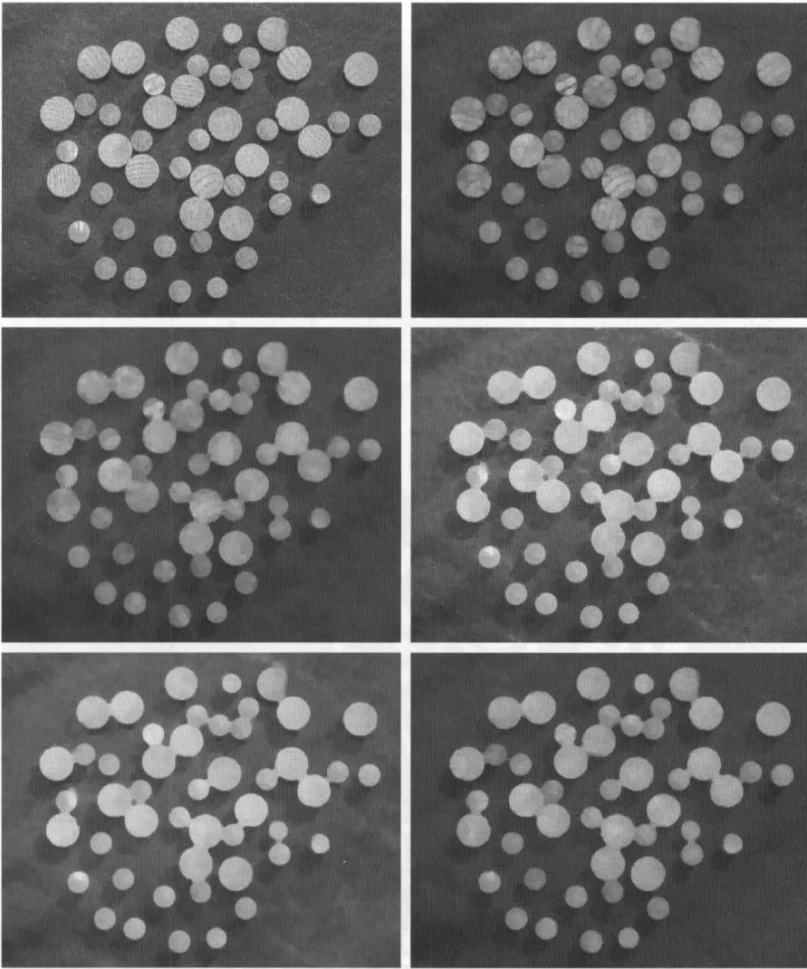
FIGURE 10.25 Smoothing using openings and closings. (a) Original image of wood dowel plugs. (b) Image opened using a disk of radius 5. (c) Closing of the opening. (d) Closing of the original image. (e) Opening of the closing. (f) Result of alternating sequential filter.
