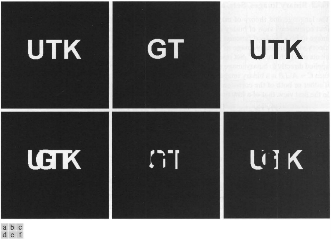
FIGURE 10.3 (a) Binary image A. (b) Binary image B. (c) Complement \neg A . (d) Union A \cup B . (e) Intersection A \cap B . (f) Set difference A \setminus B .
