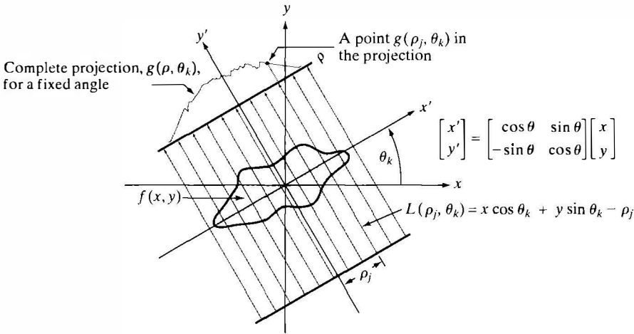
FIGURE 5.14 Geometry of a parallel-ray beam and its corresponding projection.
