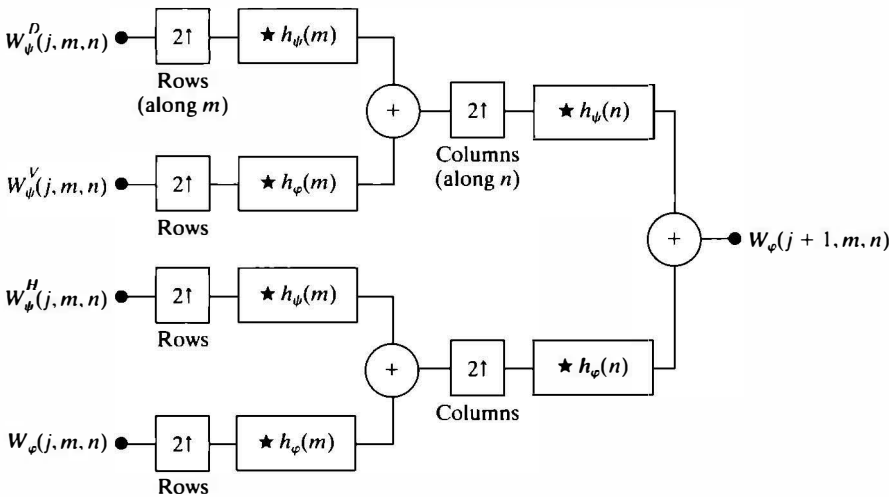
FIGURE 8.6 The 2-D FWT -1 filter bank. The boxes with the up arrows represent upsampling by inserting zeroes between every element.
