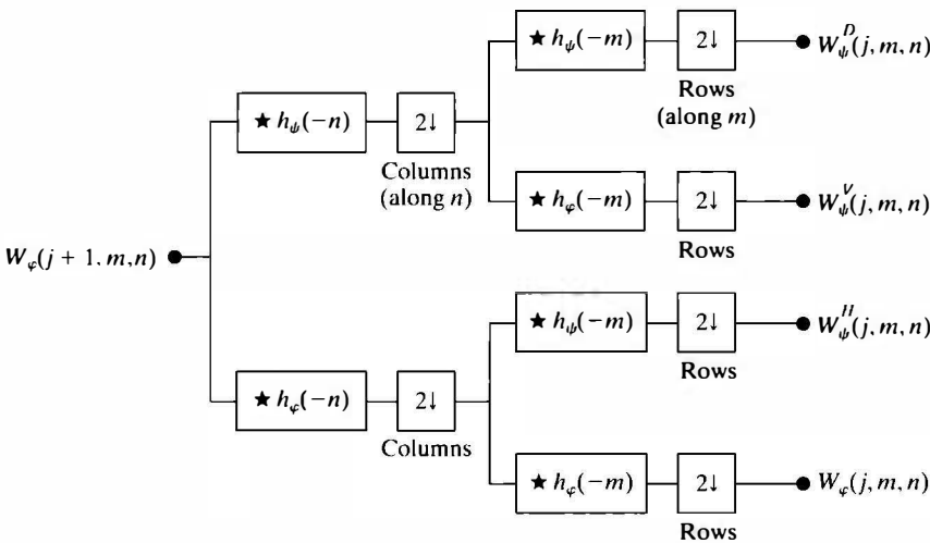
FIGURE 8.2 The 2-D fast wavelet transform (FWT) filter bank. Each pass generates one DWT scale. In the first iteration, W_\varphi(j + 1, m, n) = f(x, y) .
