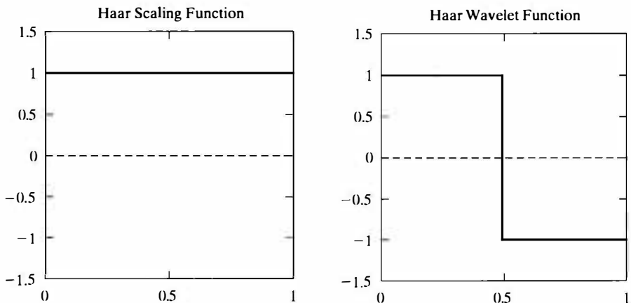
FIGURE 8.3 The Haar scaling and wavelet functions.
