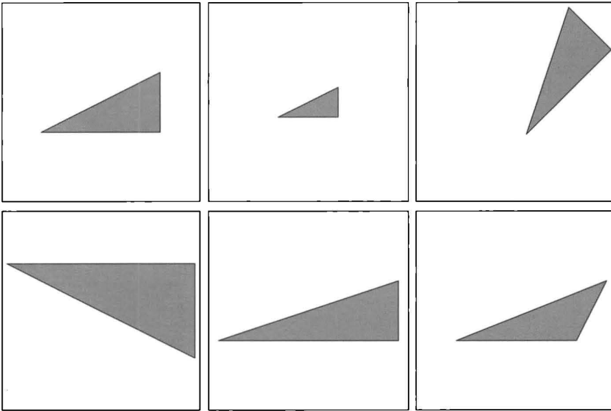
FIGURE 6.4 Examples of similarity transformations. (a) Original object. (b) Scaled. (c) Rotated and translated. (d) Reflected and scaled. (e) Scaled horizontally but not vertically—not a similarity. (f) Horizontal shearing—not a similarity.
