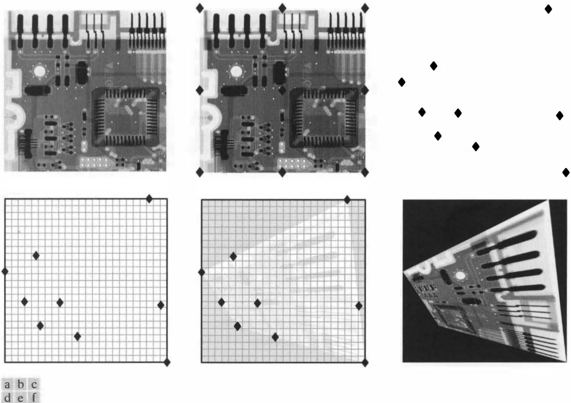
FIGURE 6.12 (a) Original image. (b) Point grid along edges and in center of image. (c) Transformed point grid. (d) Bounding box of transformed point grid, with output pixel grid. (e) Output image pixels computed inside automatically-determined output pixel grid. (f) Final result.
