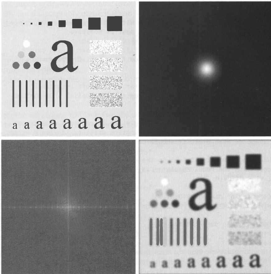
FIGURE 4.13 Lowpass filtering. (a) Original image. (b) Gaussian lowpass filter shown as an image. (c) Spectrum of (a). (d) Filtered image.
