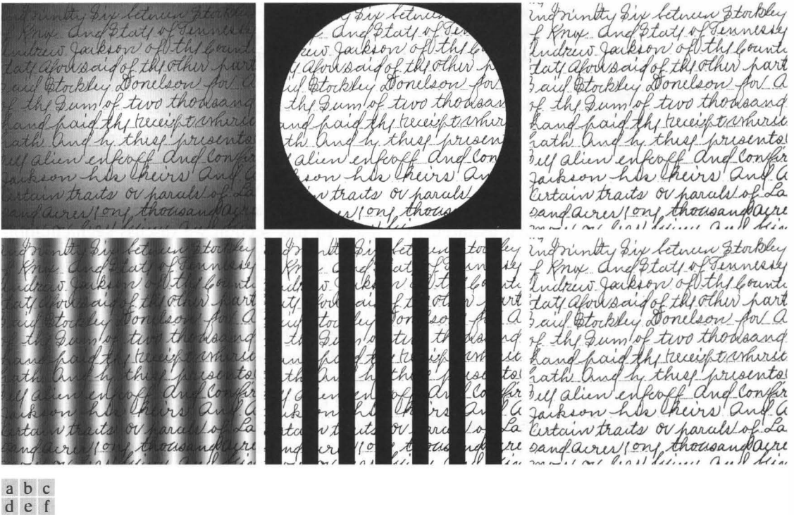
FIGURE 11.19 (a) Text image corrupted by spot shading. (b) Result of global thresholding using Otsu's method. (c) Result of local thresholding using moving averages. (d)–(f) Results of using the same sequence of operations on an image corrupted by sinusoidal shading.
