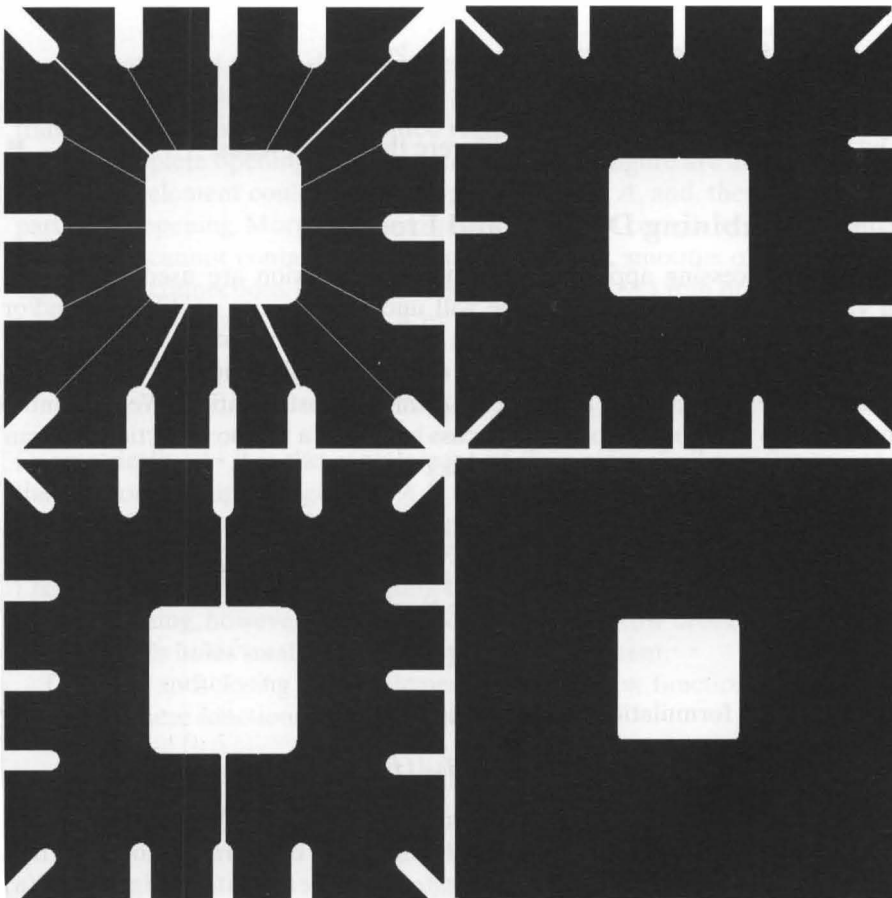
FIGURE 10.8 An illustration of erosion. (a) Original image of size 486 \times 486 pixels. (b) Erosion with a disk of radius 10. (c) Erosion with a disk of radius 5. (d) Erosion with a disk of radius 20.
