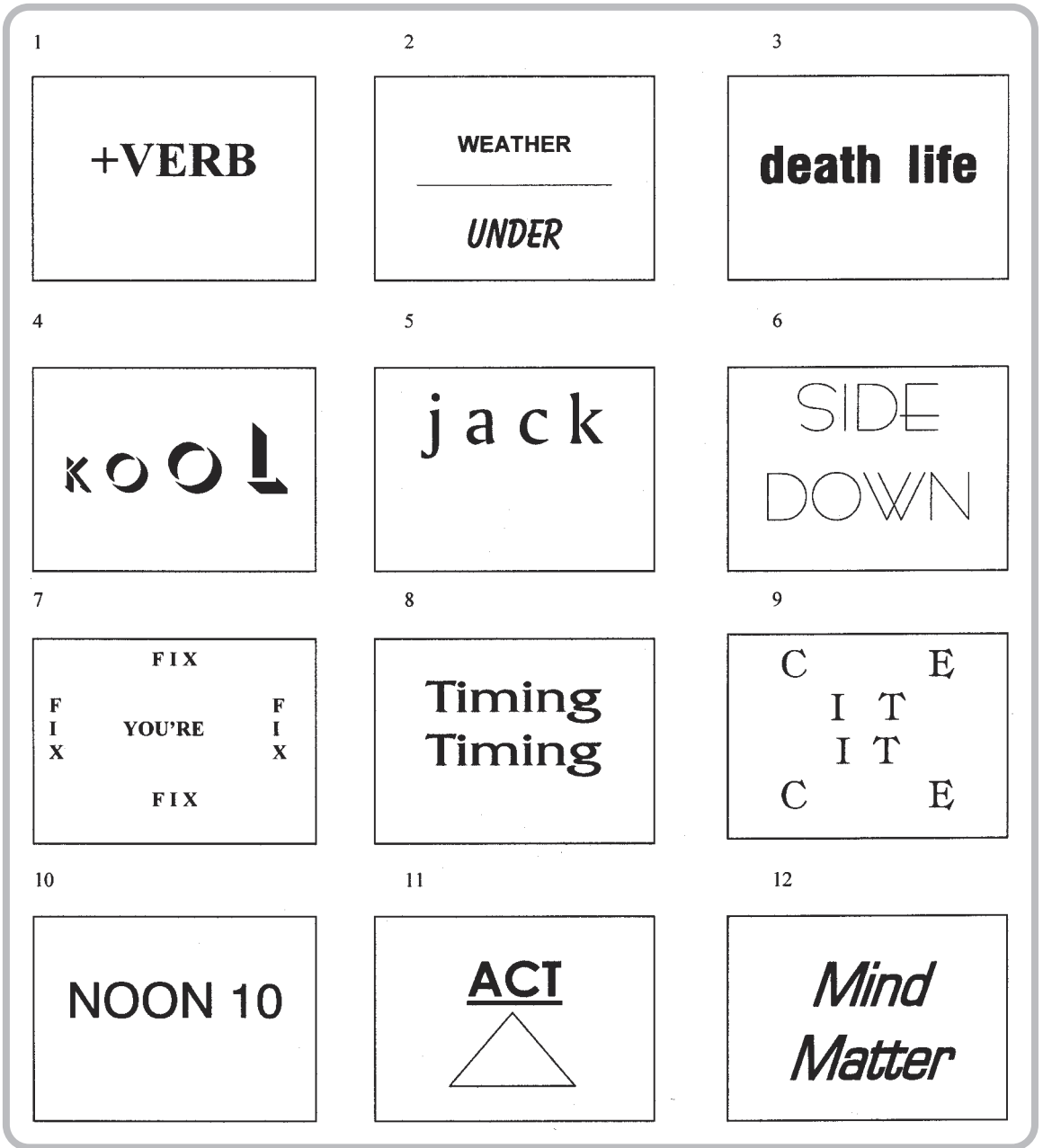
FIGURE 4-7. Brain teaser
