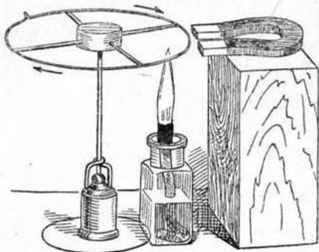
142. ROTATION OF A RING BEFORE A MAGNET.
