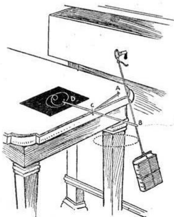
61. THE CONICAL PENDULUM.
