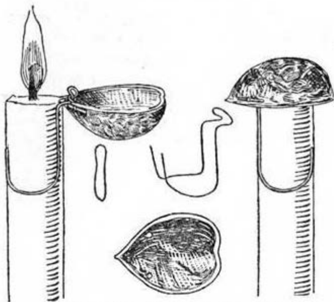
150. THE AUTOMATIC EXTINGUISHER.
