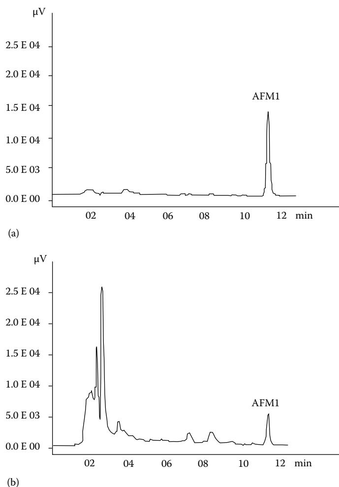
Figure 33.3 LC-FLD chromatograms of (a) AFM1 standard solution at 0.004 \mu\text{g/mL} ; (b) naturally contaminated pasteurized milk with an AFM1 concentration of 0.004 \mu\text{g/L} . (Reprinted from Zinedine, A. et al., Int. J. Food Microbiol. , 114, 25, 2007. With permission.)
