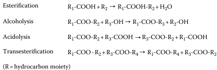
Figure 20.2 Lipolytic enzymes catalyze a variety of reactions. (Adapted from Holland, R. et al., Int. Dairy J. , 15, 711, 2005. With permission.)
