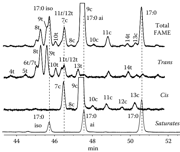
Figure 9.5 Partial gas chromatograms of milk fat separated using a GC program at 150°C depicting the 16:1 FA isomers. The total milk FAMES were compared with the trans , cis , and saturated FA fractions isolated from total milk fat FAMES using Ag + -SPE columns. (From Kramer, J.K.G. et al., Lipids , 43, 259, 2008. With permission.)
