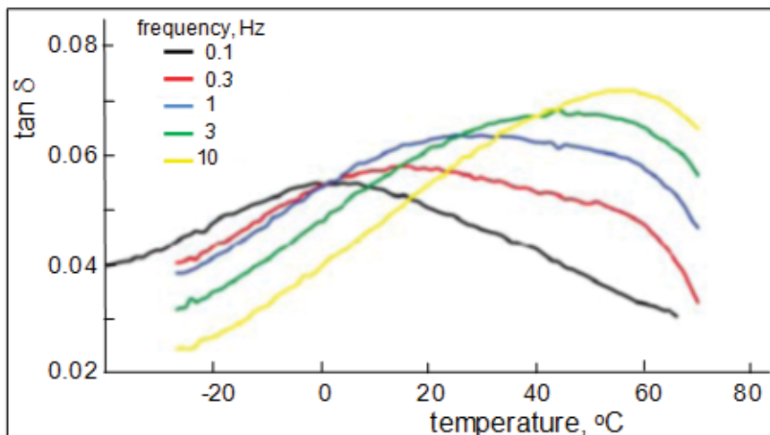
Figure 7.10 Tan δ vs. temperature at various frequencies over the β-transition of PMMA (source: PerkinElmer-1)
