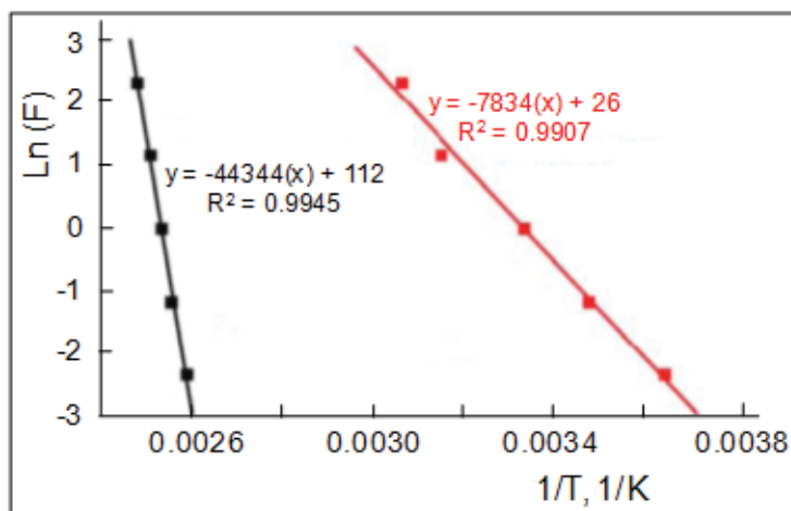
Figure 7.11 Arrhenius plots for (■) β and (■) α transitions of PMMA (source: PerkinElmer-1)
