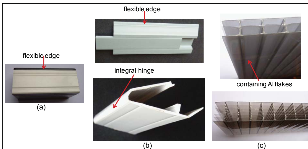
Figure 3.38 Sections of various extruded and co-extruded profiles: (a) U-PVC bus/coach interior trimming (b) a two-part and integral-hinge U-PVC skirting board for homes, caravans and auto-homes, and (c) structured-PC roofing for conservatories/gazebos
