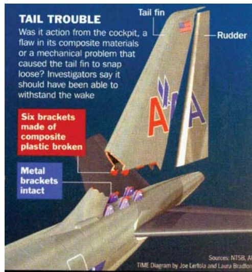
Figure 6.23 Illustration of the aircraft tail section failure at the November 2001 crash (source: TIME, November 26, 2001)
