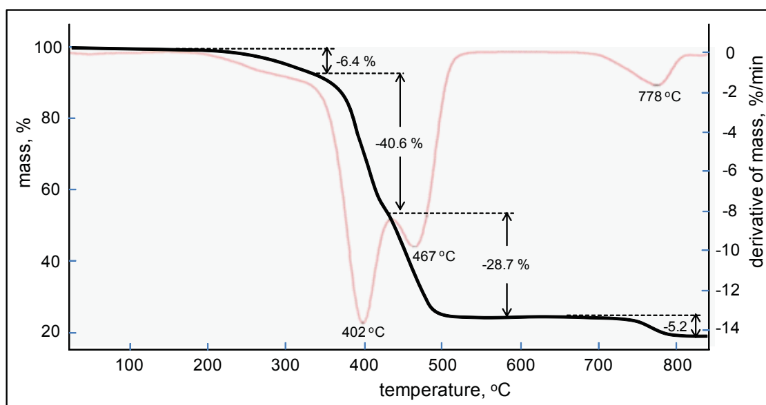
Figure 7.5 (–) TGA and (–) DTG traces for a blend of natural and SBR rubber (source: Netzsch GmbH (see Reference (Kaisersberger 1994))
