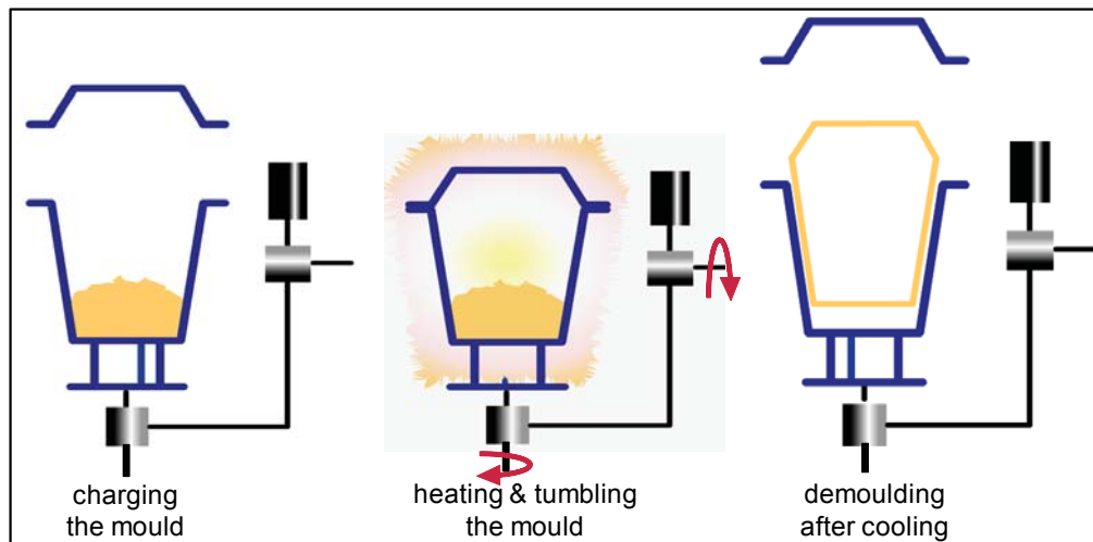
Figure 3.44 Illustration of rotational moulding
