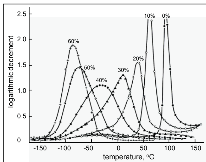
Figure 7.27 Logarithmic decrement at 1 Hz vs. temperature for PVC plasticised with diethylhexyl succinate at concentrations (by volume) indicated on the curves (source: Schmieider & Wolf 1952)
