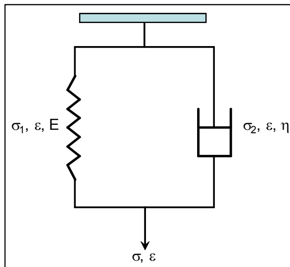
Figure 5.3 Voigt model, subjected to stress ( \sigma ) and strain ( \epsilon )
