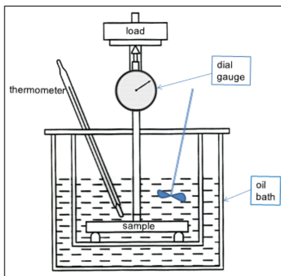
Figure 7.29 HDT test set up
