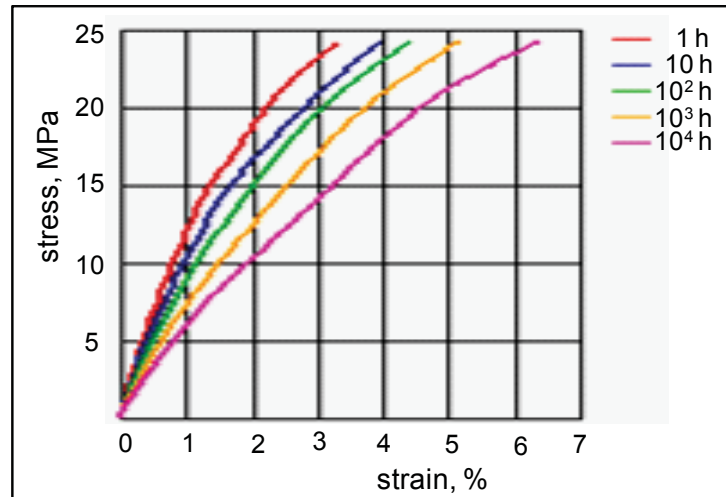
Figure 6.12 \sigma - \varepsilon isochronous curves for Zytel 101L NC010 (PA66) (cond.) at 23 °C
